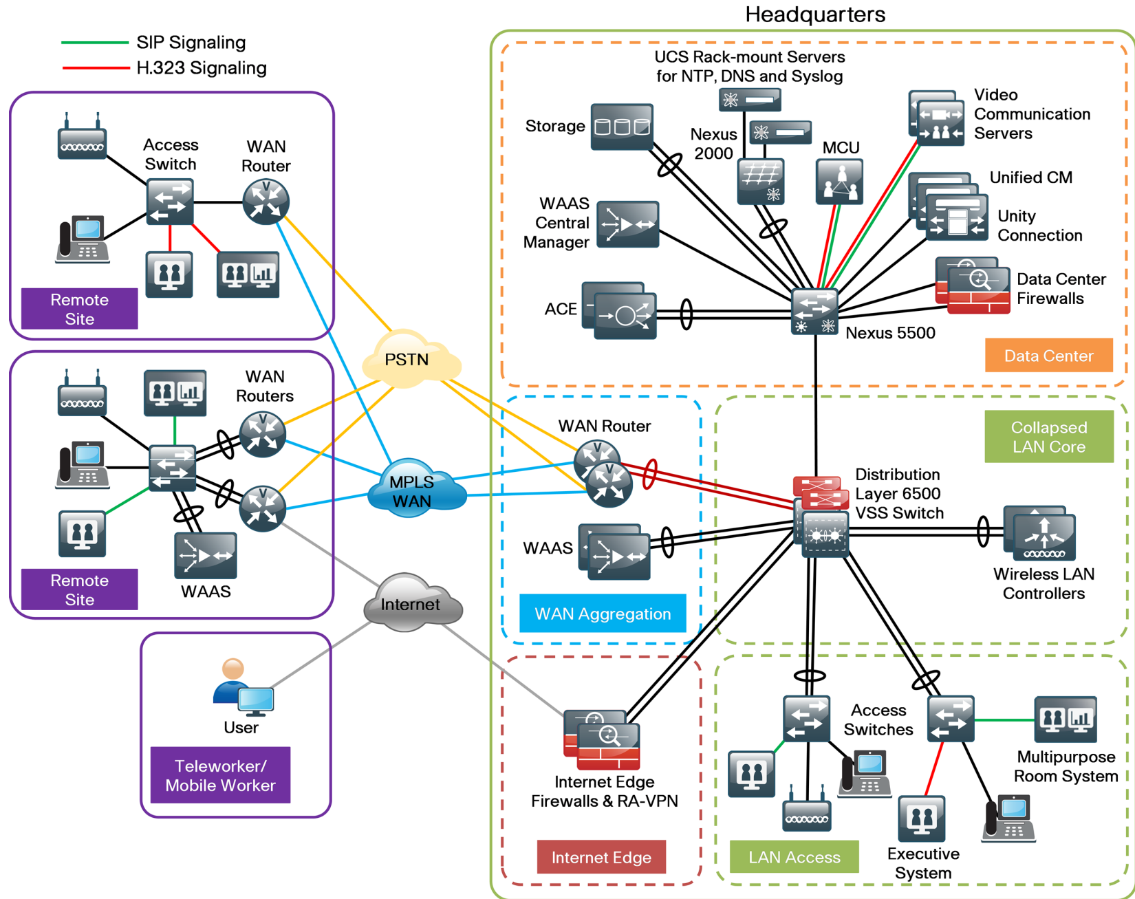
Figure 1 - SIP and H.323 video room systems in the Cisco SBA foundation
