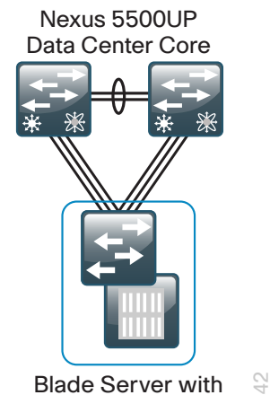
Figure 24 - Third-party blade server system with integrated switch
