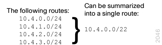
Figure 2 - Route summarization
