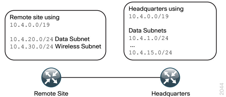
Figure 5 - Overlapping IP address space, non conflicting
