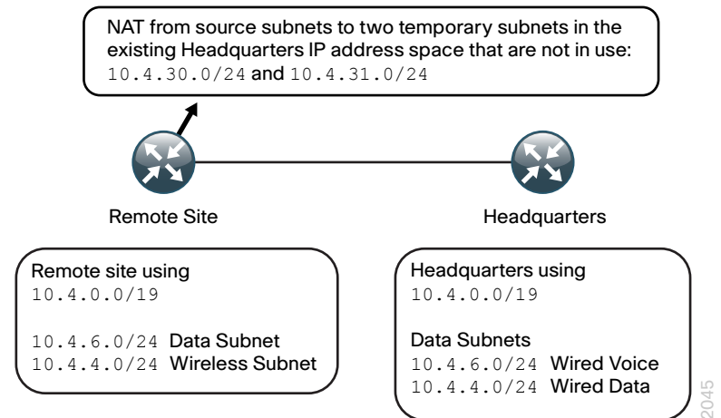
Figure 6 - Overlapping IP address space, conflicting
