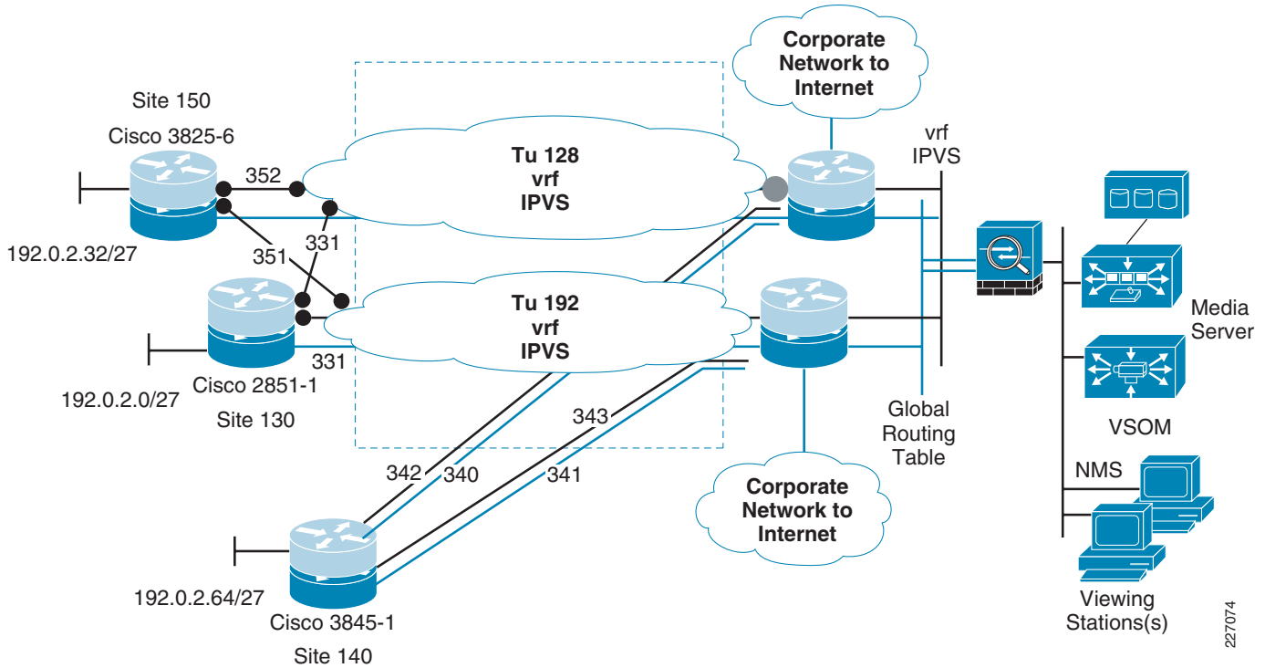
Figure 3 Virtualization Topology
