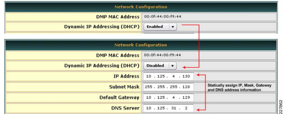
Figure 15 Assigning DMP Static IP Address
