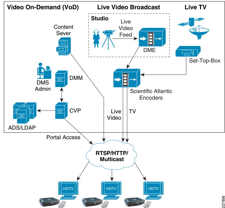
Figure 4 Live Video Broadcast and VoD Using Enterprise TV Application
