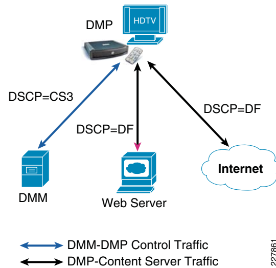
Figure 14 QoS Marking Between Digital Signage Components
