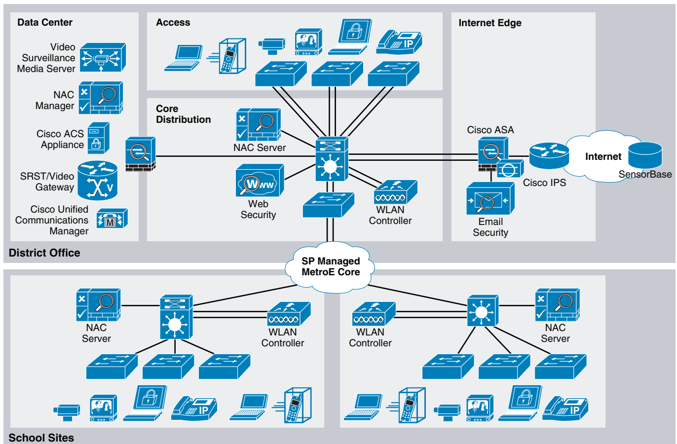
Figure 1 Secure School Design
