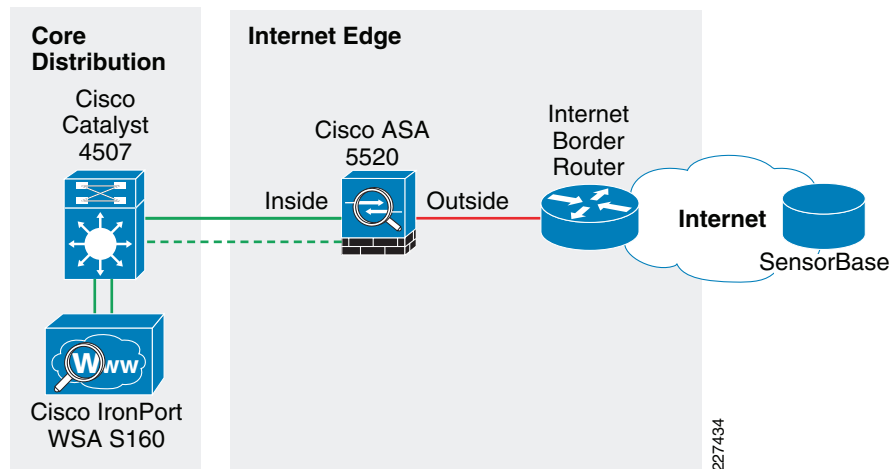
Figure 18 WSA deployment
