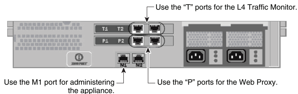
Figure 19 WSA Interfaces
