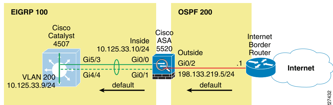
Figure 15 Cisco ASA OSPF
