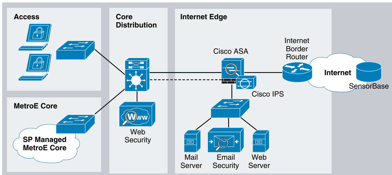
Figure 2 Internet Perimeter
