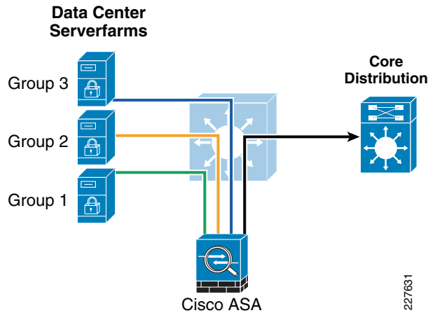
Figure 12 Service Isolation
