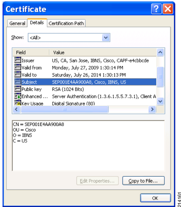
Figure 10 Sample LSC
