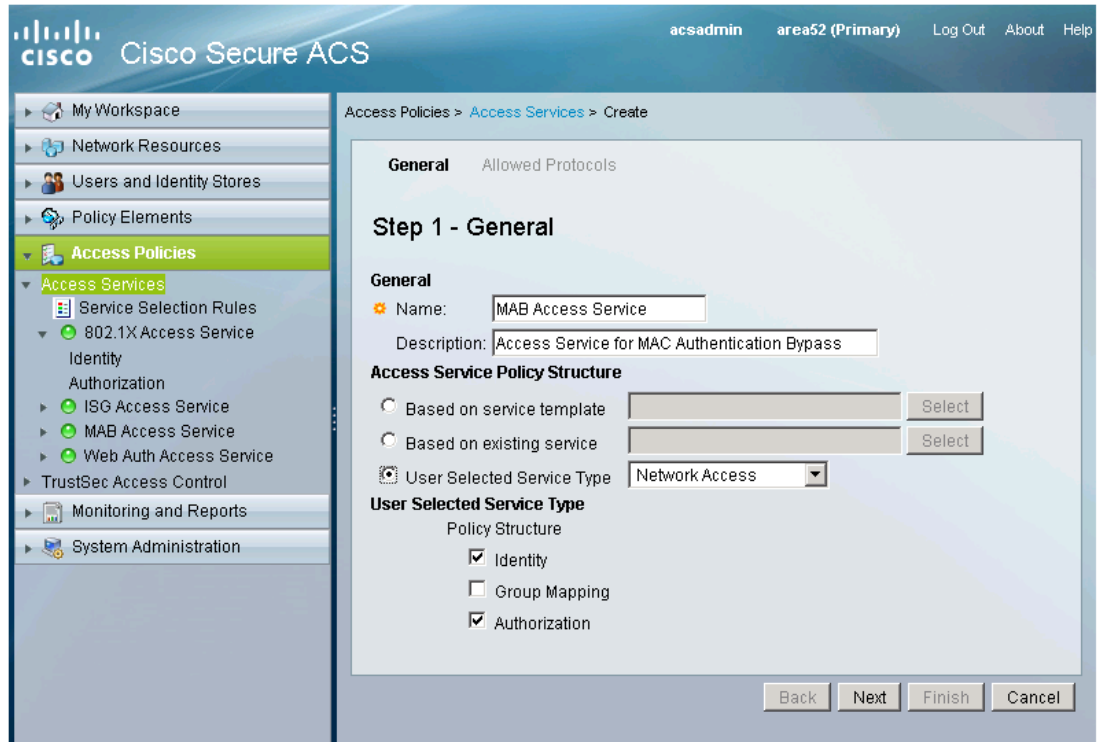
Figure 29 Access Services—General
