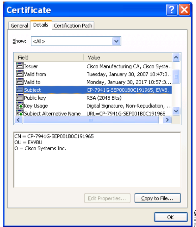
Figure 9 Sample MIC
