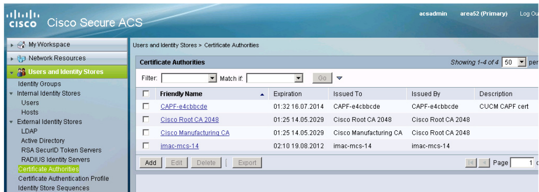
Figure 18 Certificate Authorities
