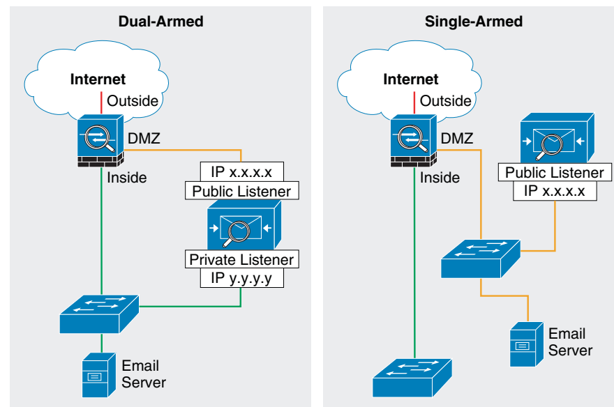
Figure 7 Common ESA Deployments
