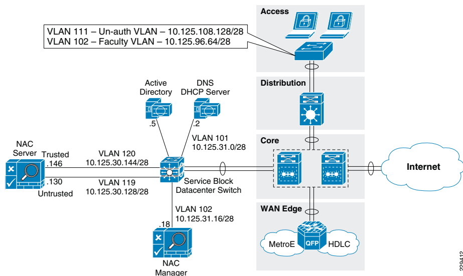
Figure 44 NAC L3 OOB Logical Topology Diagram
