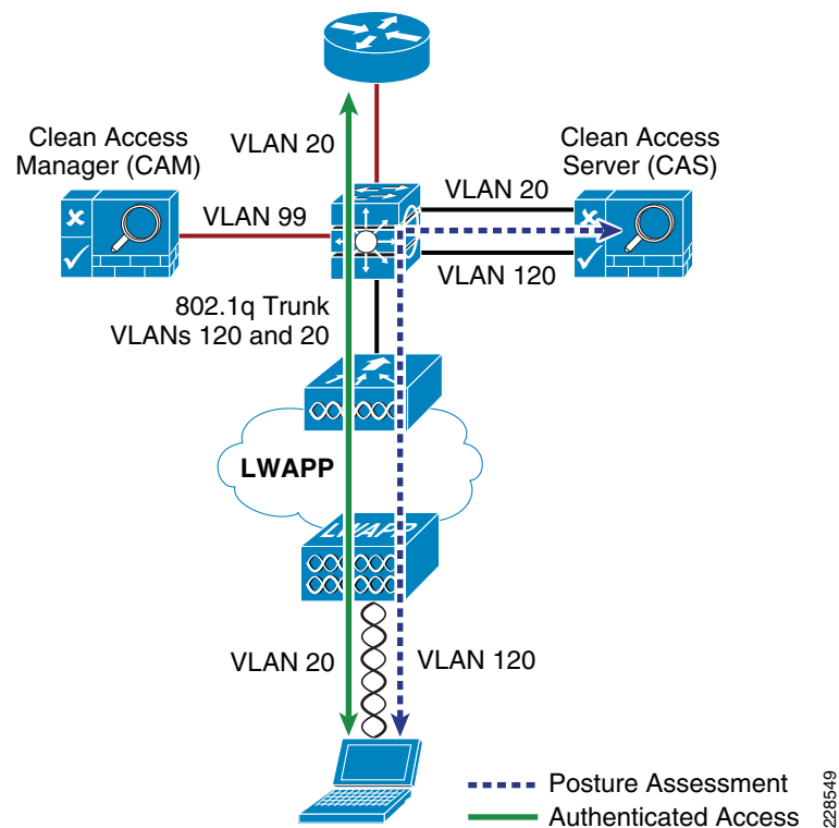
Figure 21 Wireless NAC OOB Traffic Flow
