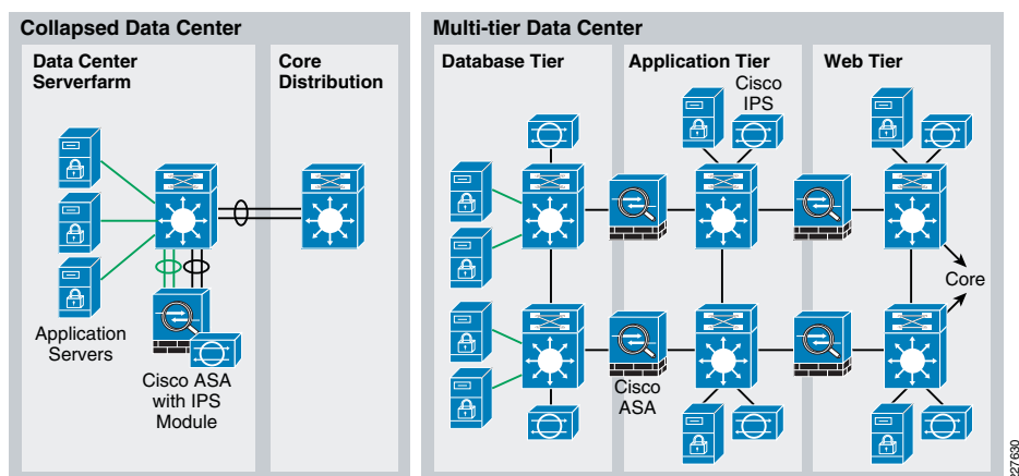
Figure 12 Collapsed and Multi-tier Data Center Designs
