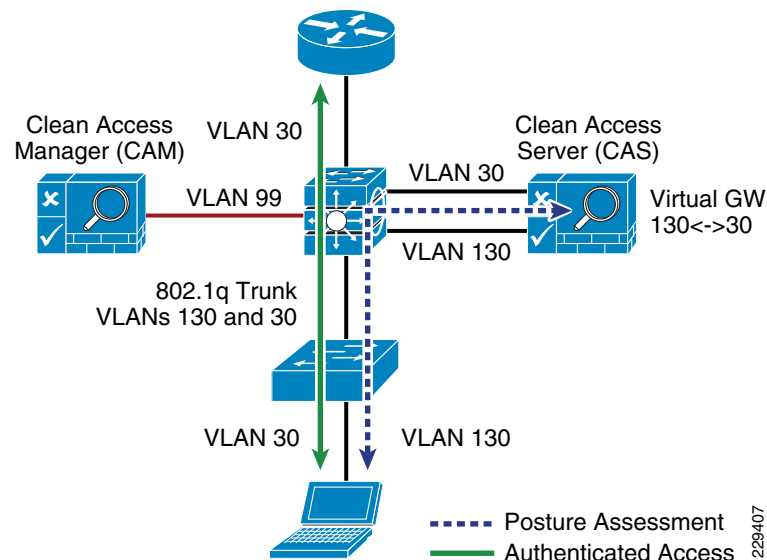
Figure 22 Layer 2 OOB Topology
