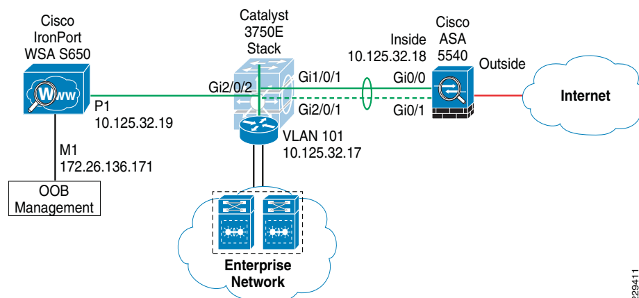
Figure 34 WSA Network Topology
