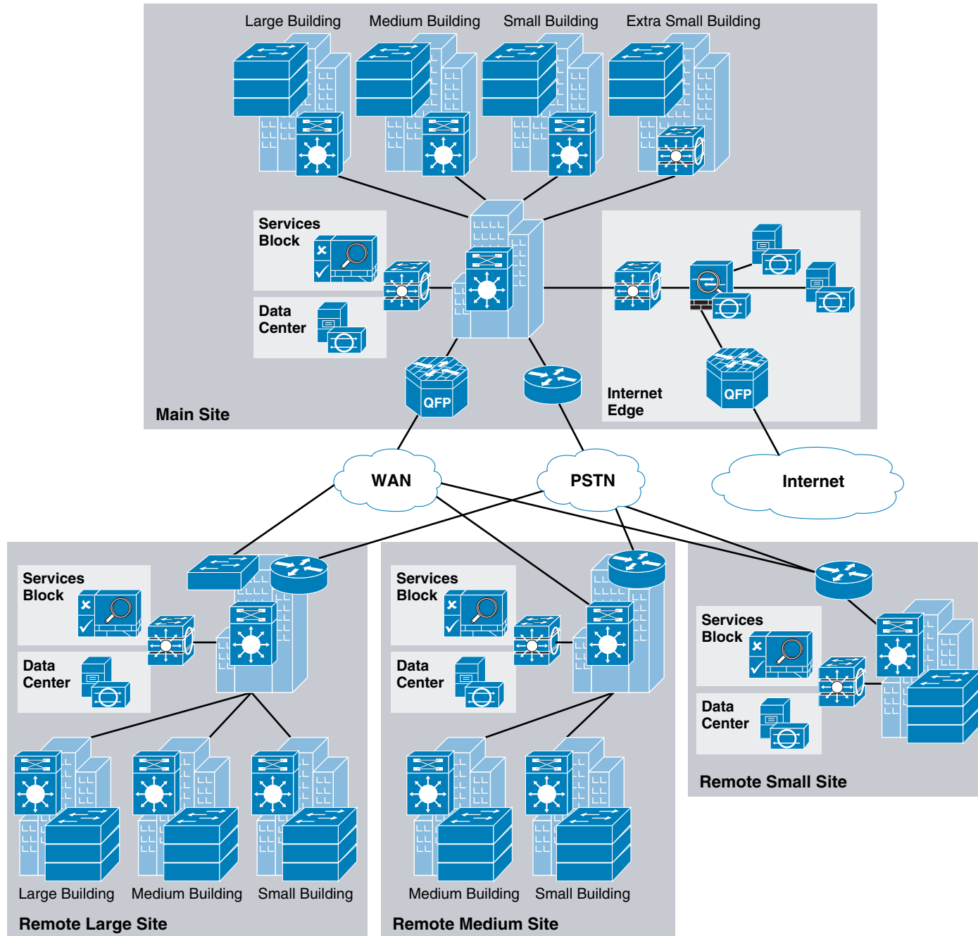
Figure 2 Medium Enterprise Design Profile Network Overview
