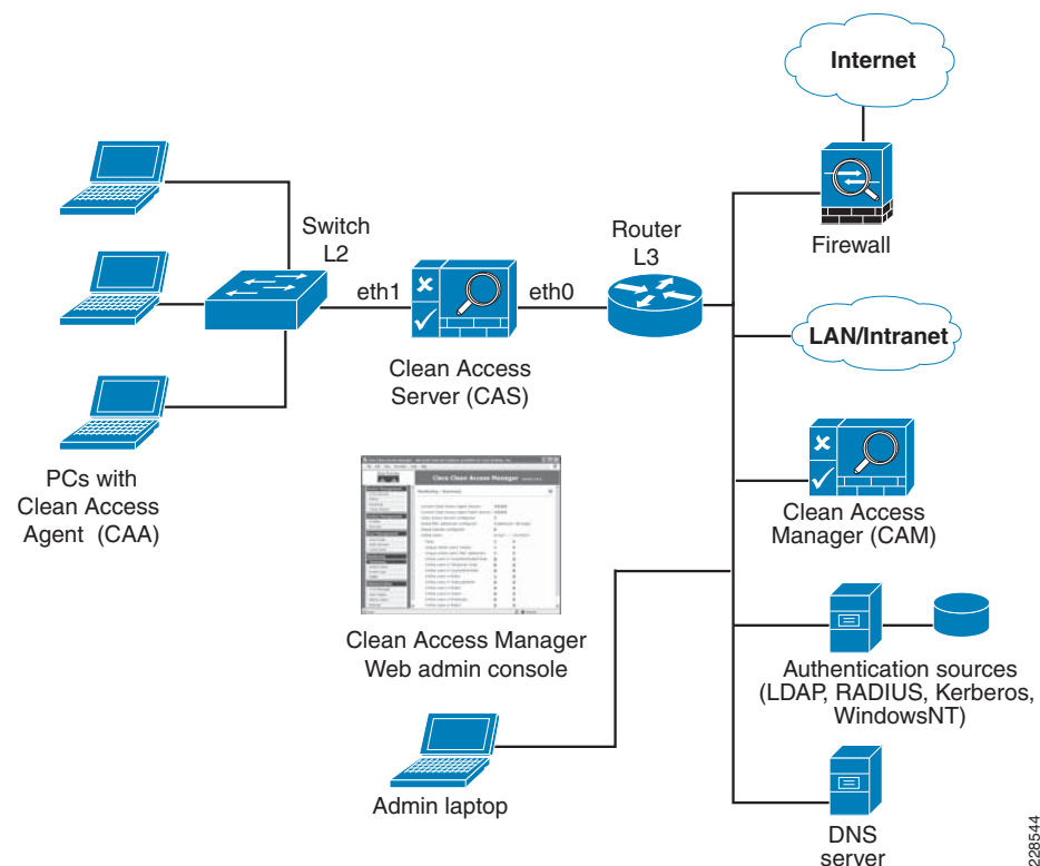
Figure 16 NAC Appliance Components
