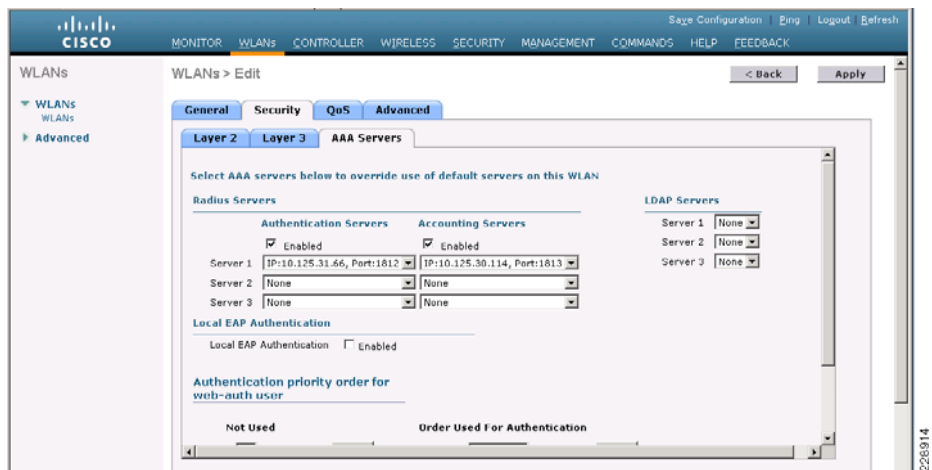
Figure 73 Enabling RADIUS Accounting for VPN SSO
