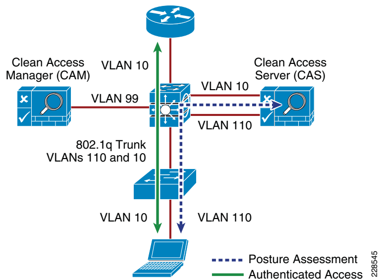
Figure 17 Layer 2 OOB Topology
