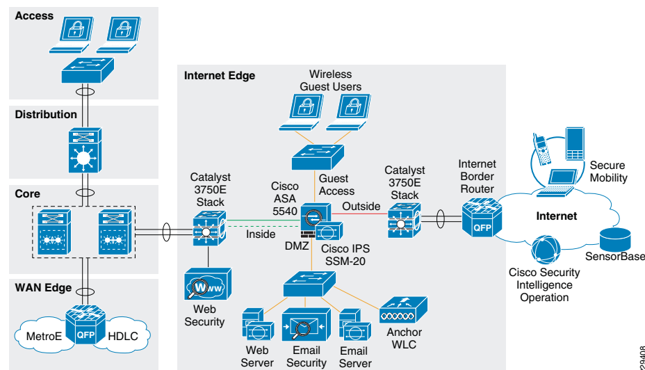
Figure 24 Internet Edge Firewall
