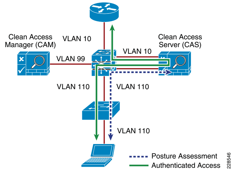
Figure 19 Physical In-Band Topology
