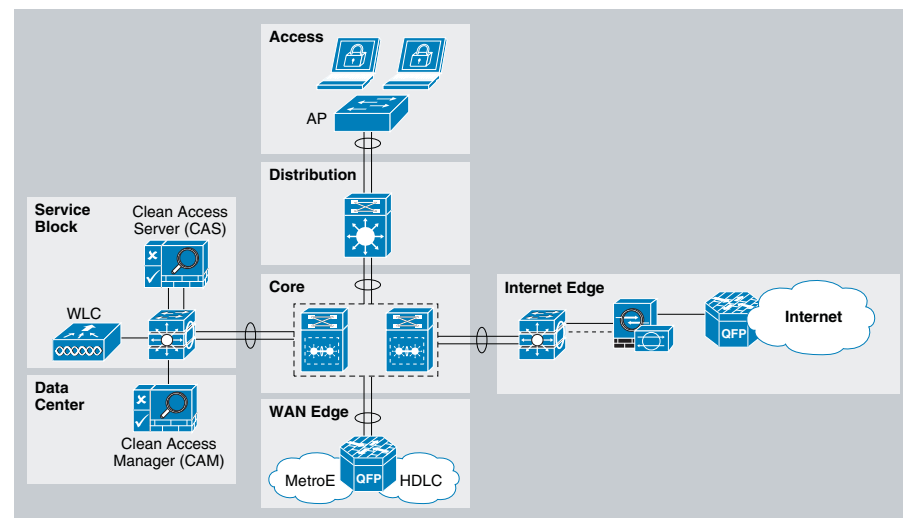
Figure 20 NAC OOB Deployment for Wireless Clients
