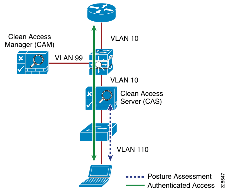
Figure 19 Physical In-Band Topology
