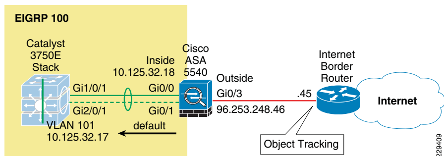
Figure 26 Cisco ASA Static Route
