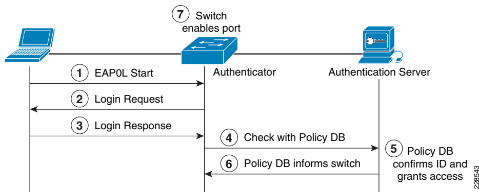
Figure 14 Port-Based Access Control
