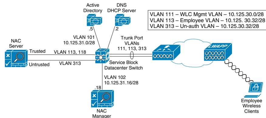
Figure 58 Layer-2 OOB NAC Deployment Topology for Employee Wireless Clients
