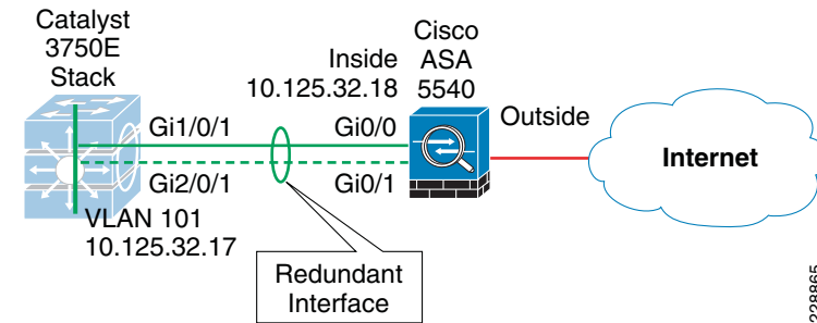
Figure 25 Cisco ASA Redundant Interface
