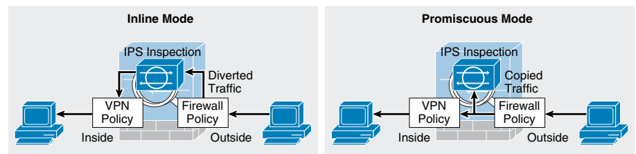
Figure 5 IPS Inline and Promiscuous Modes
