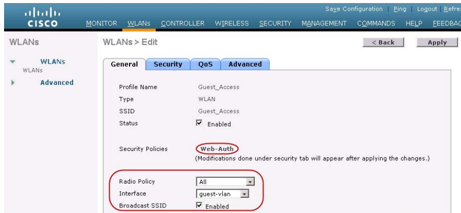
Figure 35 Anchor WLAN Controller Interfaces
