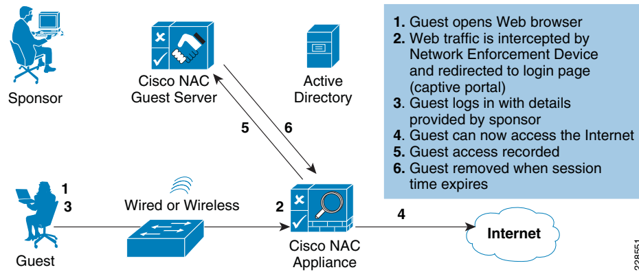
Figure 16 NAC Guest Server with NAC Appliance and WLAN Controller
