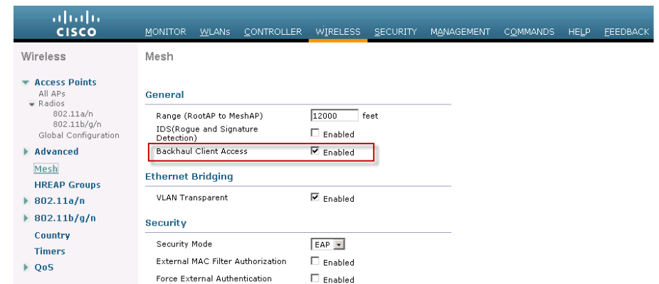
Figure 42 Enabling Backhaul Client Access
