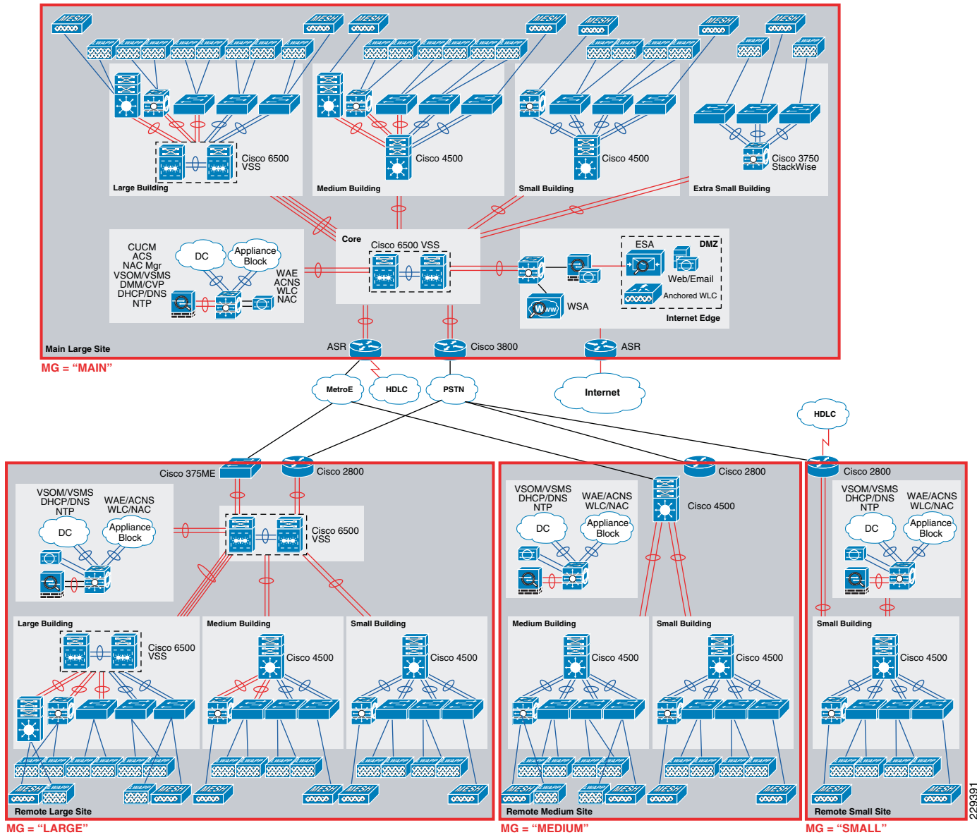
Figure 9 Medium Enterprise Mobility Groups
