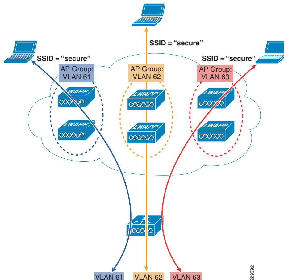
Figure 10 Access Point (AP) Groups
