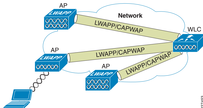
Figure 4 CAPWAP Access Point to WLC Communication
