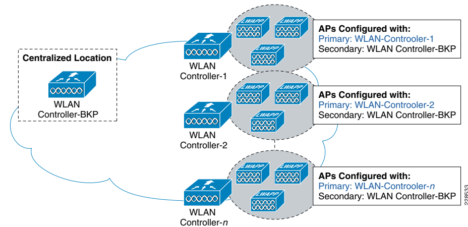
Figure 21 General N+1 WLAN Controller Redundancy
