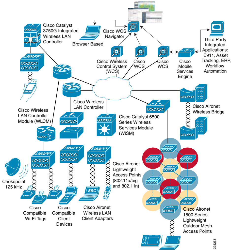
Figure 2 Cisco Unified Wireless Network Overview
