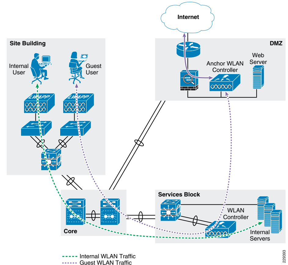
Figure 14 Guest Access Solution High-Level Overview
