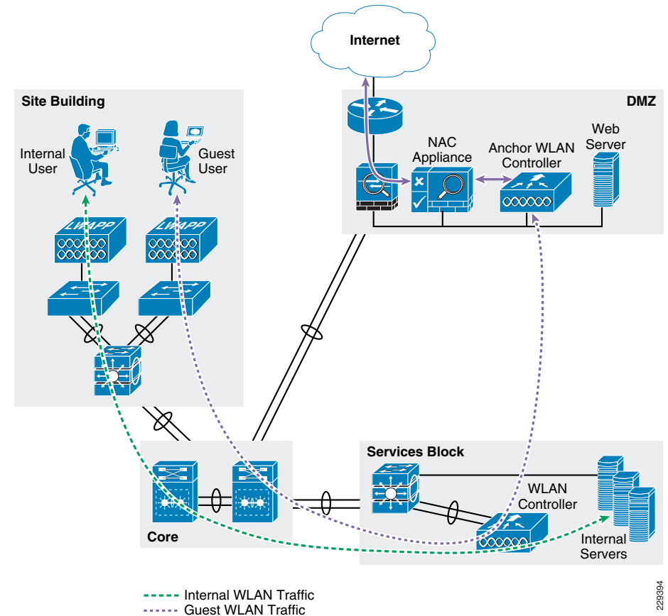
Figure 15 Cisco UWN Guest Access with Anchor WLC and NAC Appliance
