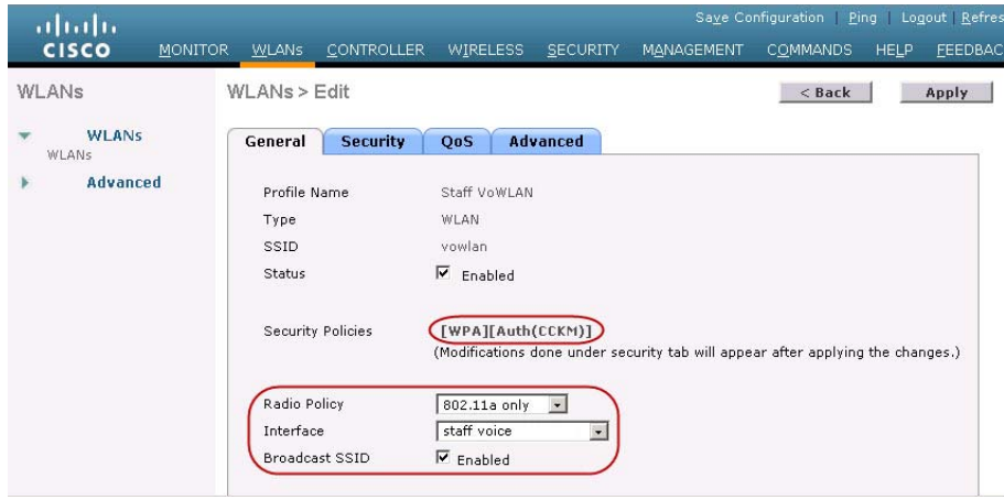
Figure 30 Staff Voice WLAN
