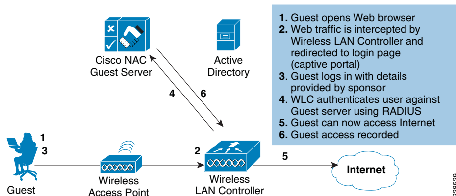
Figure 17 NAC Guest Server with WLAN Controller Alone
