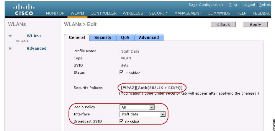
Figure 29 Staff Data WLAN
