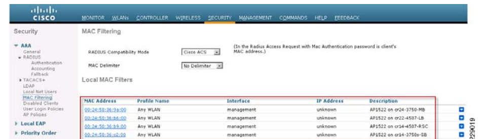
Figure 40 Adding the AP1520 MAC Address to the WLAN Controller
