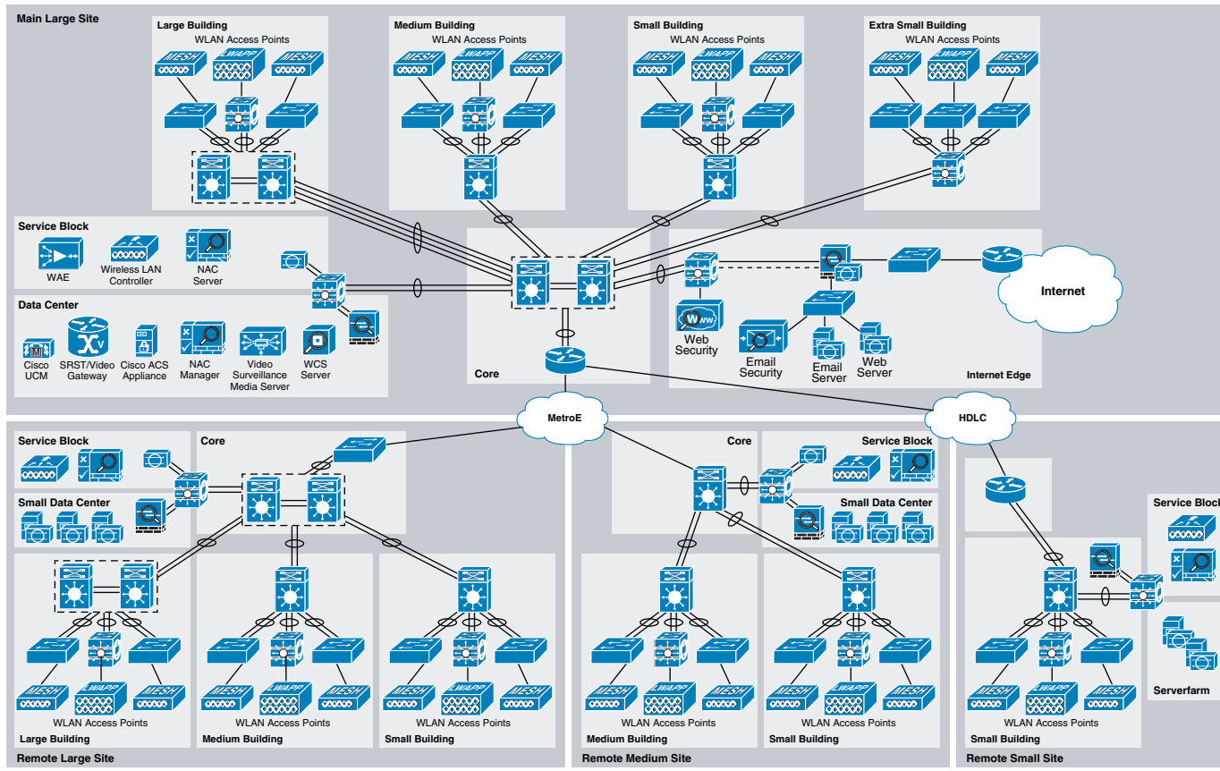
Figure 3 Medium Enterprise Design Profile Overview
