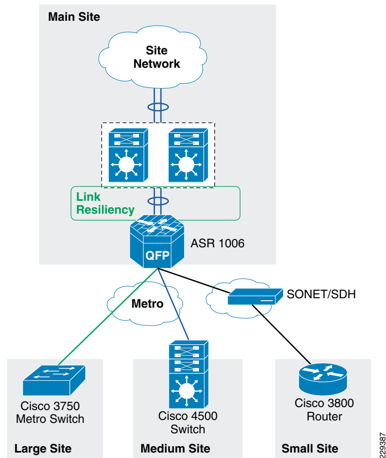
Figure 17 Link Resiliency
