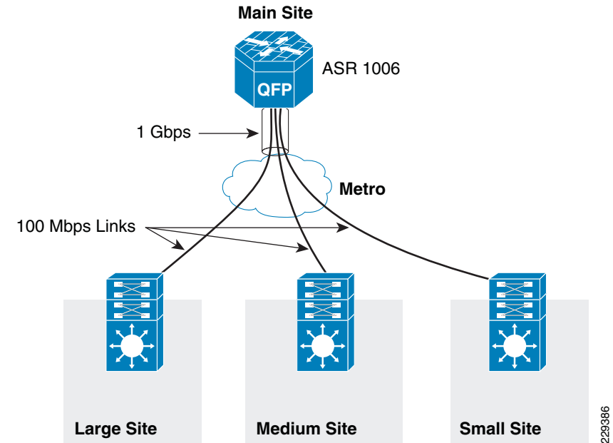
Figure 16 The WAN Link Design for Connectivity Between Main Site and Medium Remote Site
