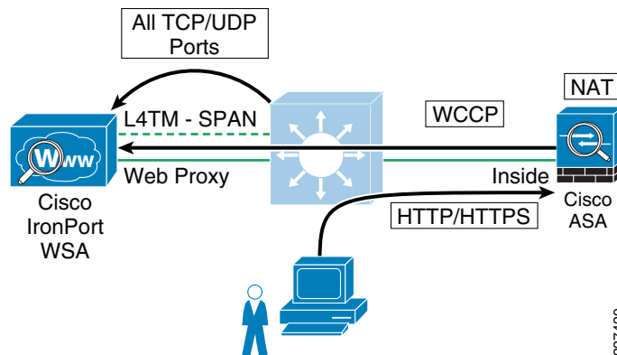
Figure 4-10 L4TM Deployment
