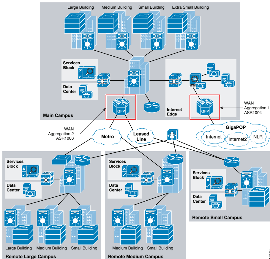
Figure 7 The WAN Aggregation Points in Community College
