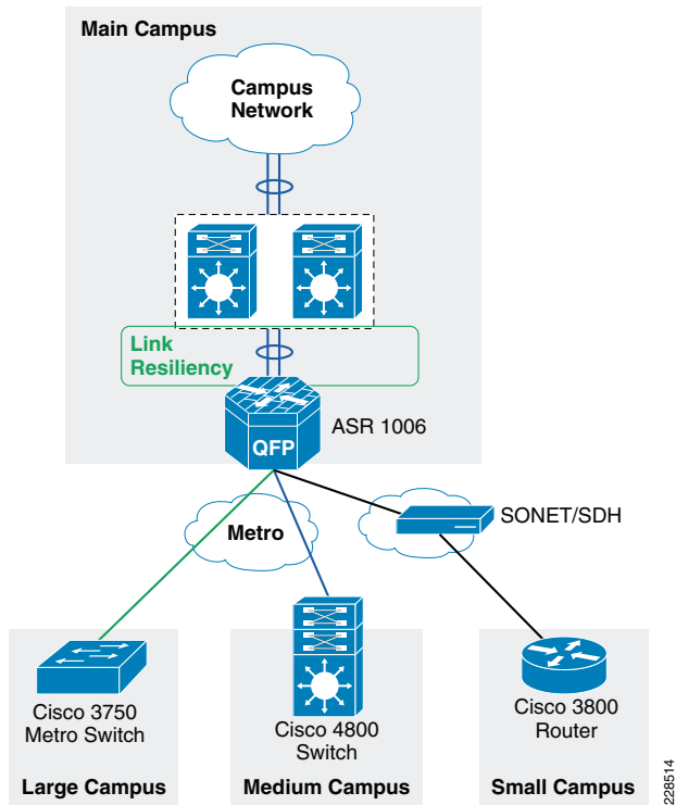
Figure 1-12 Link Resiliency
