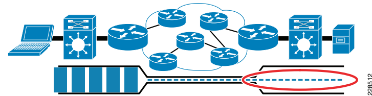
Figure 10 Bandwidth Constraint Due to Difference in Speeds
