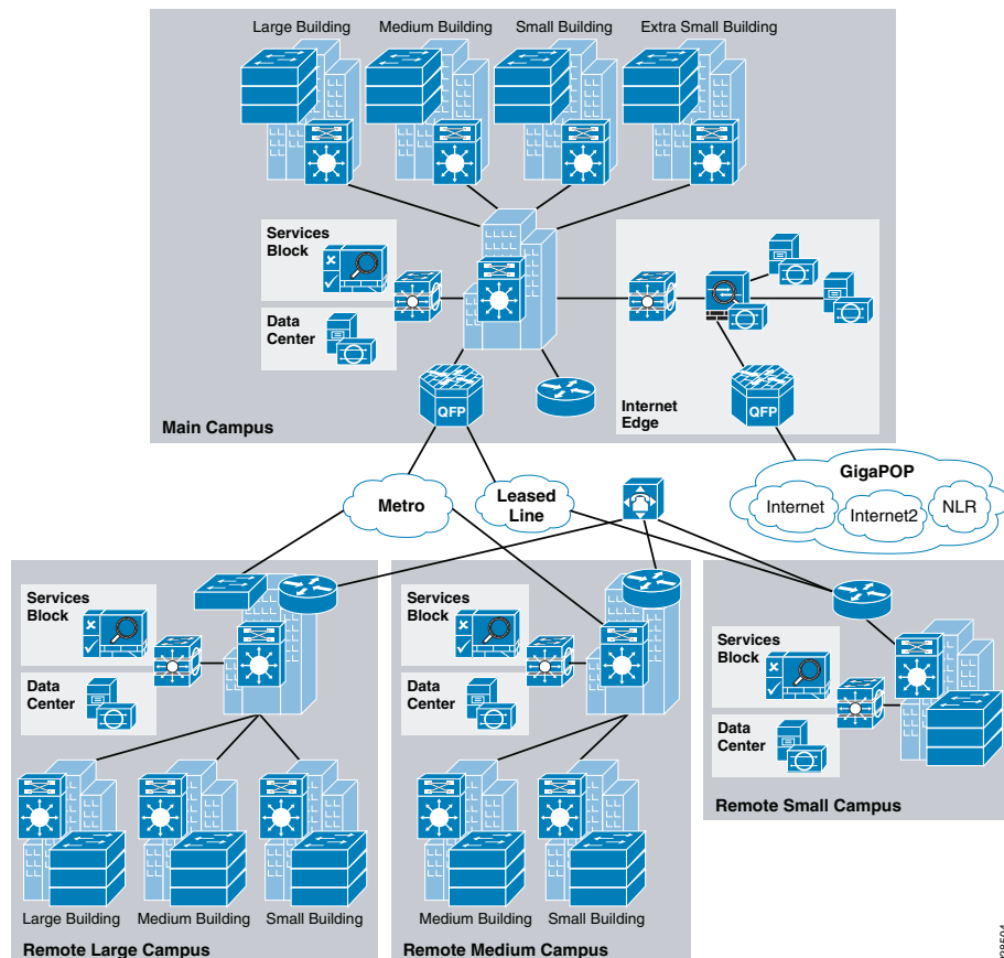
Figure 1 Community College WAN Design Diagram
