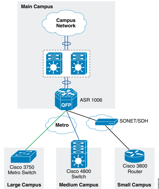
Figure 6 The Metro Transport Deployment in Community College WAN Design
