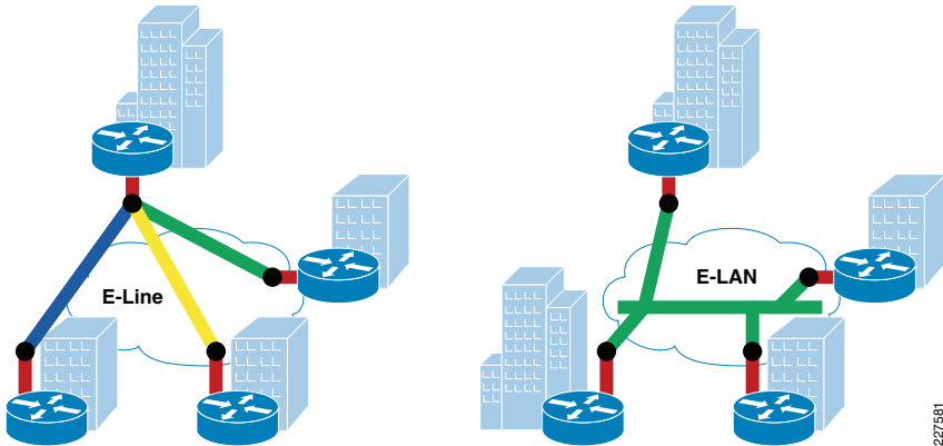
Figure 5 Different Services Available
