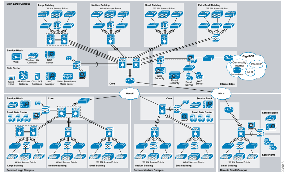
Figure 3 Community College Reference Design Overview
