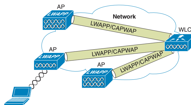
Figure 4 CAPWAP Access Point to WLC Communication
