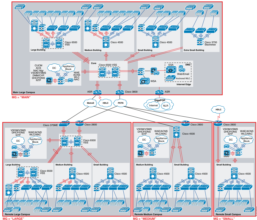
Figure 9 Community College Mobility Groups
