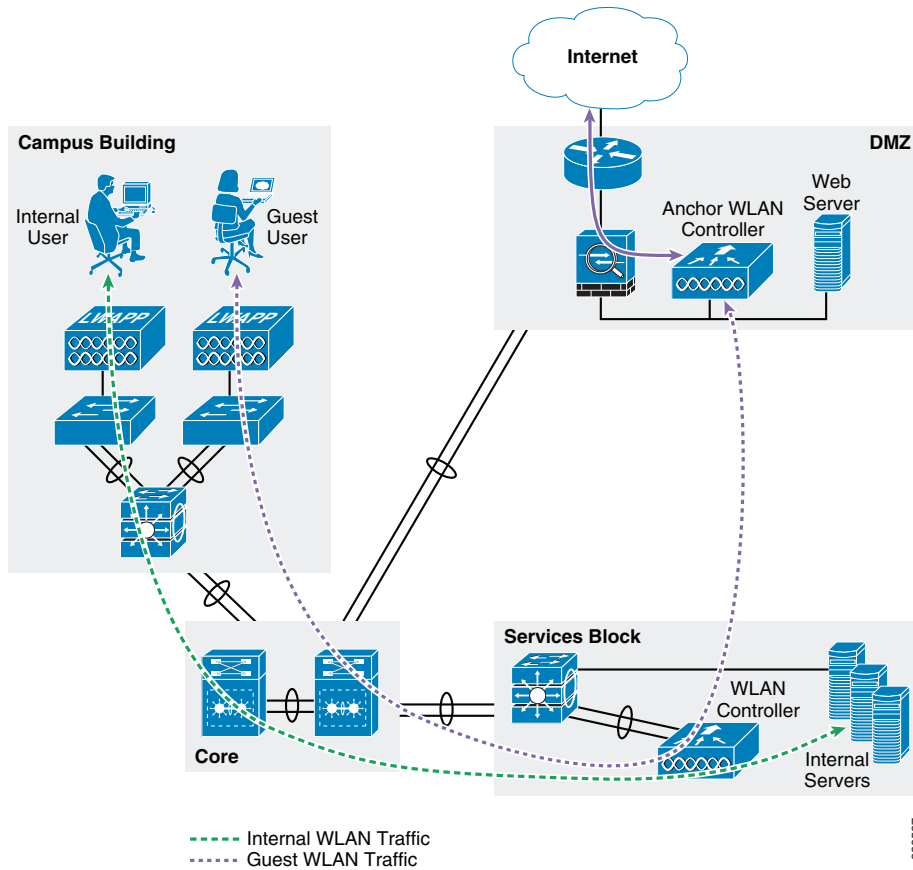
Figure 14 Guest Access Solution High-Level Overview
