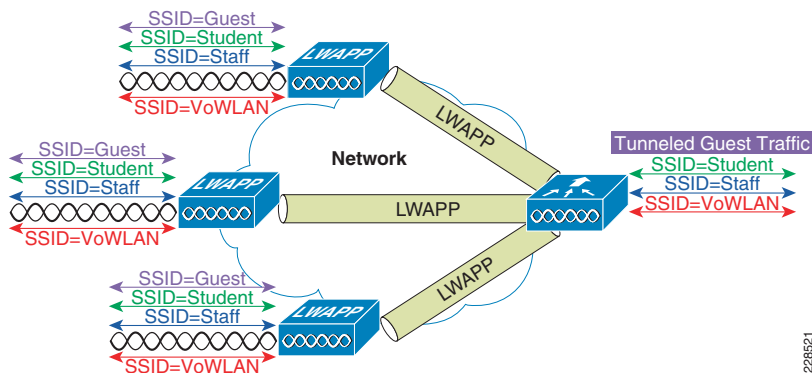
Figure 7 WLAN SSIDs
