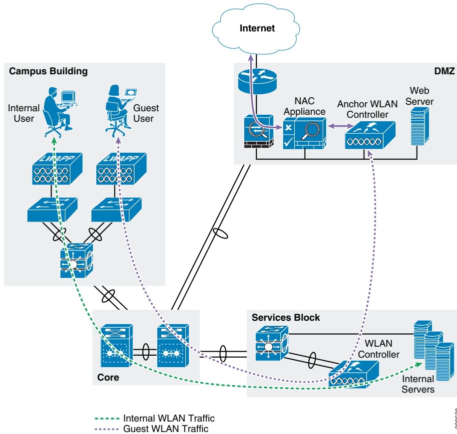
Figure 15 Cisco UWN Guest Access with Anchor WLC and NAC Appliance
