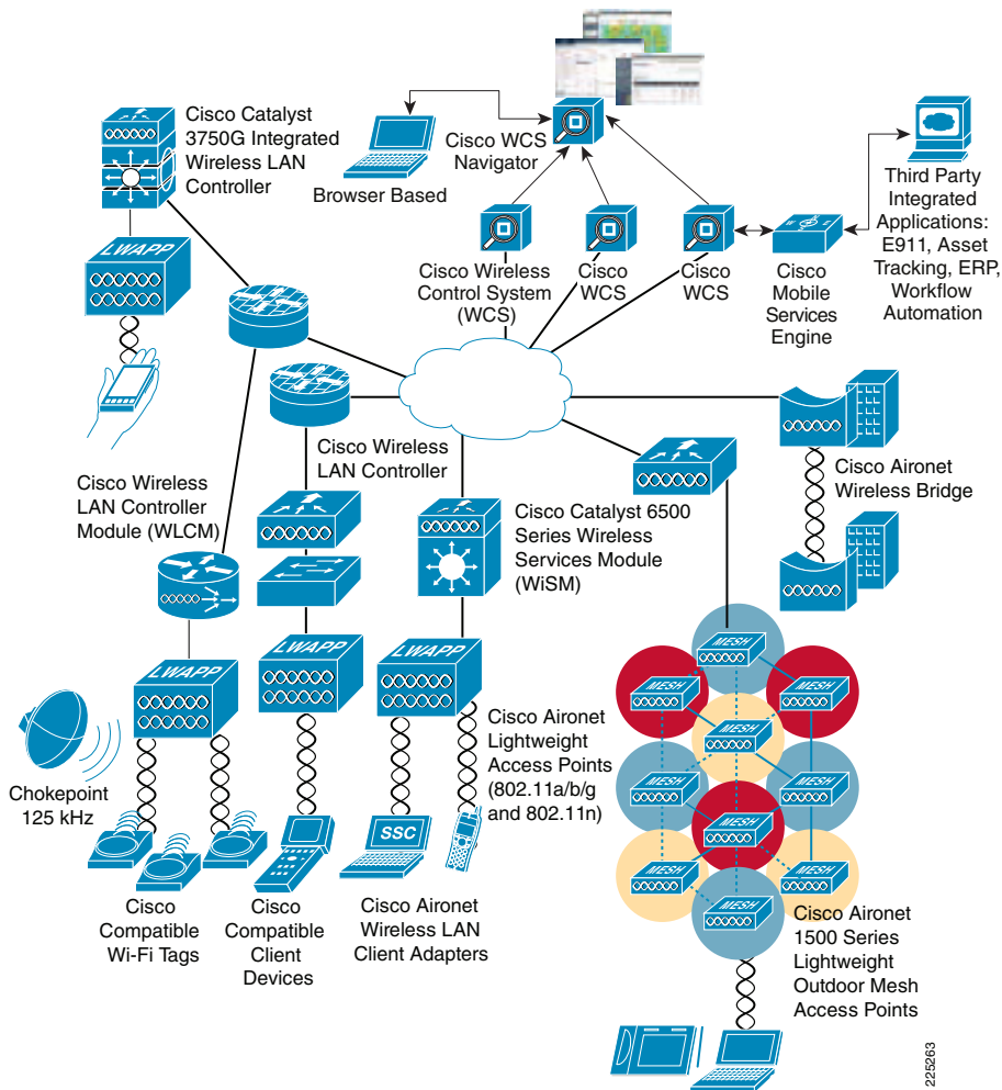
Figure 2 Cisco Unified Wireless Network Overview
