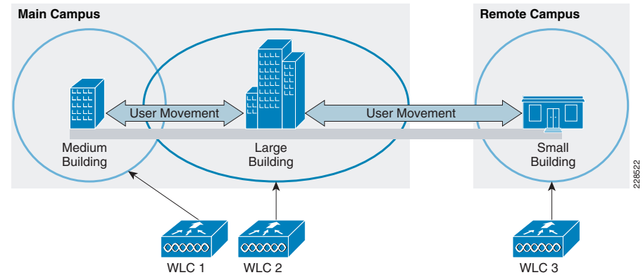
Figure 8 Campus Roaming
