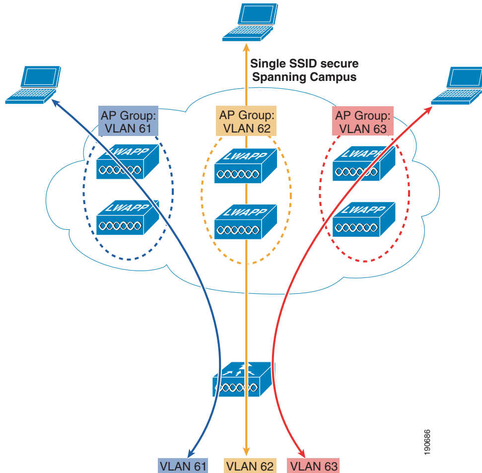
Figure 5-10 Access Point (AP) Groups
