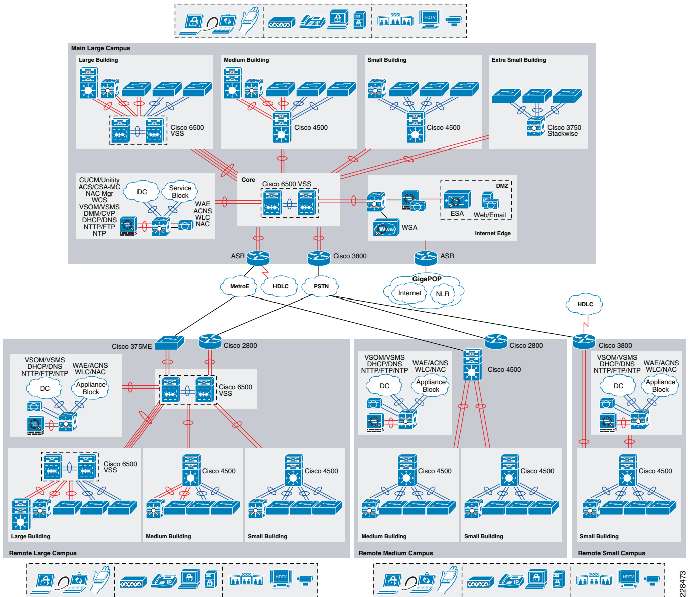
Figure 3-6 Community College LAN Design Model
