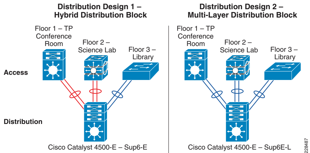
Figure 3-21 Two Cisco Catalyst 4500-E-Based Distribution Layer Options
