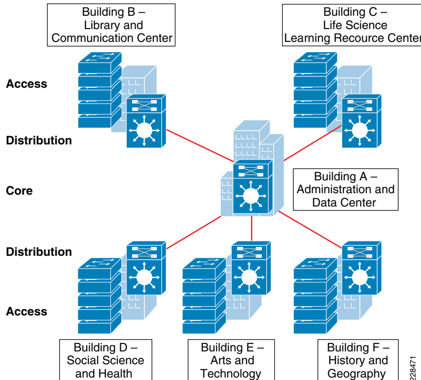
Figure 3-4 Three-Tier LAN Network Design Example
