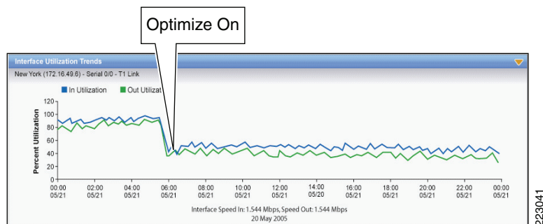
Link Utilization
