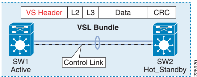
Figure 3 VSL Header and Control Link
