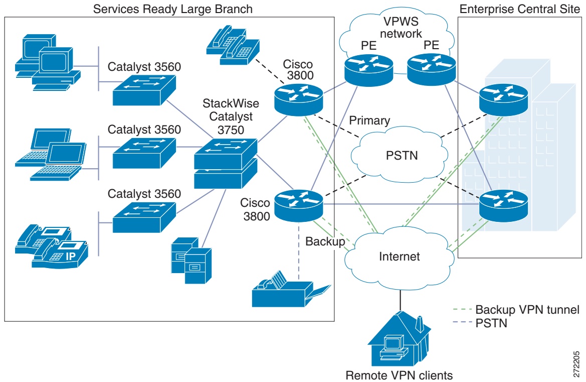
Figure 24 The Services Ready Large Branch Network VPWS Deployment
