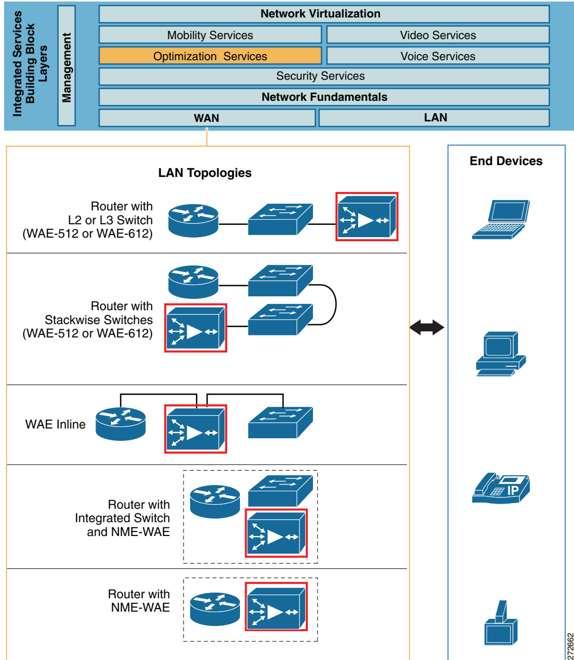
Figure 64 Cisco WAAS Deployment Options
