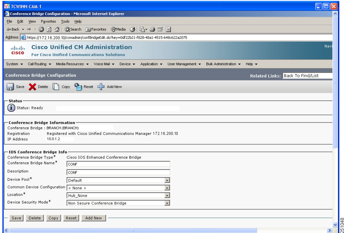
Figure 95 Conferencing Configuration for Cisco Unified SRST Mode
