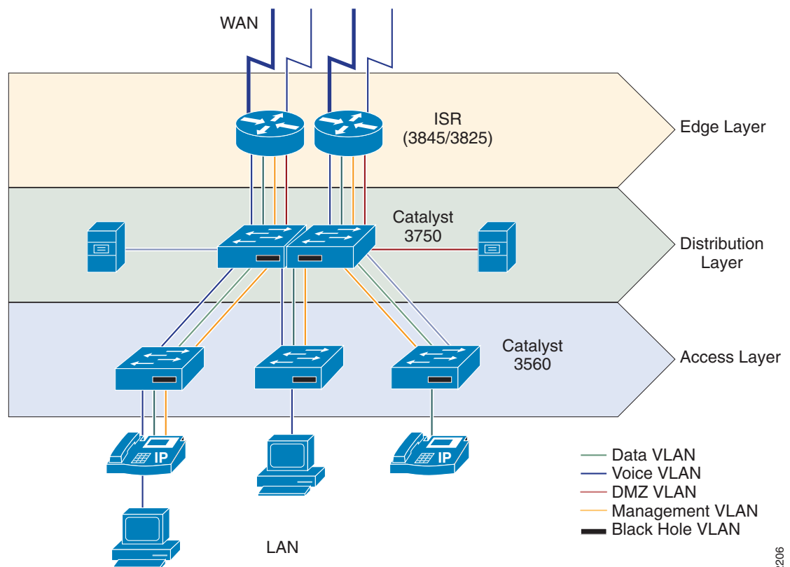
Figure 27 VLAN Design
