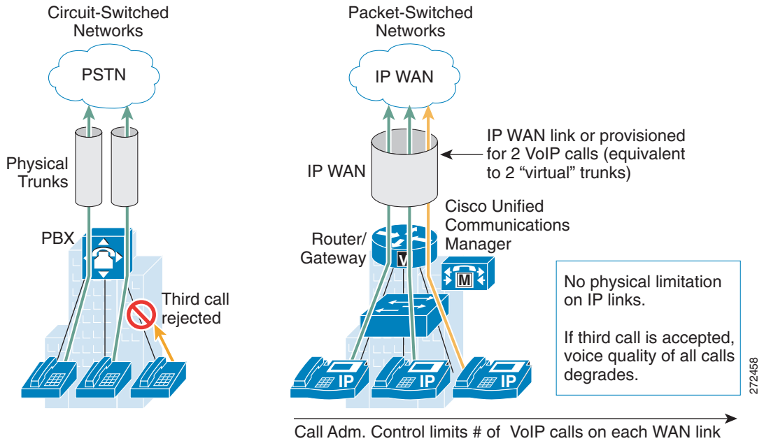
Figure 59 Traditional Versus VoIP Call Admission Control
