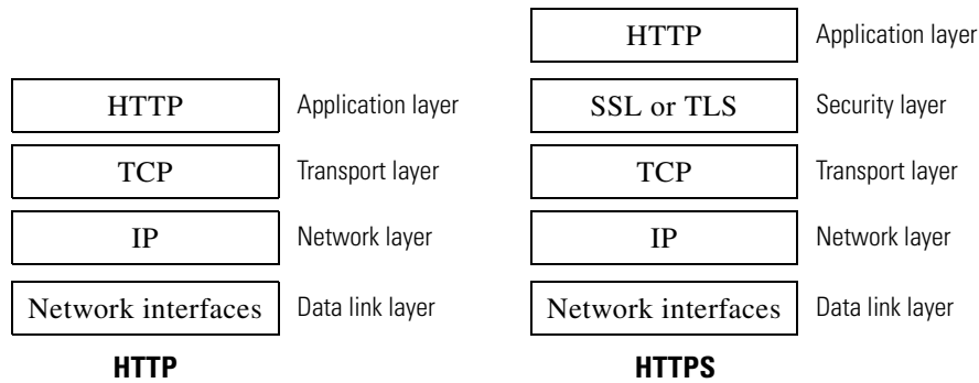
Figure 12-1 HTTPS and HTTP OSI Layers
