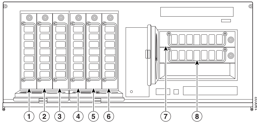
Figure 11-4 Hard Drive Slot Numbering for MARS Local Controller 200 and Global Controllers
