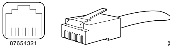
Figure A-2 RJ-45 Cable
