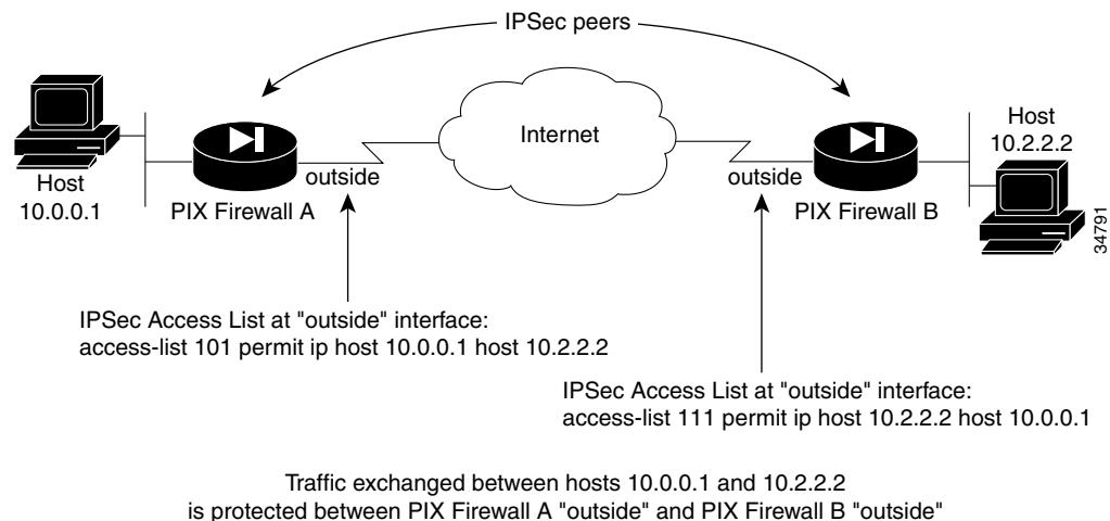
Figure 4-1 How Crypto Access Lists Are Applied for Processing IPsec
