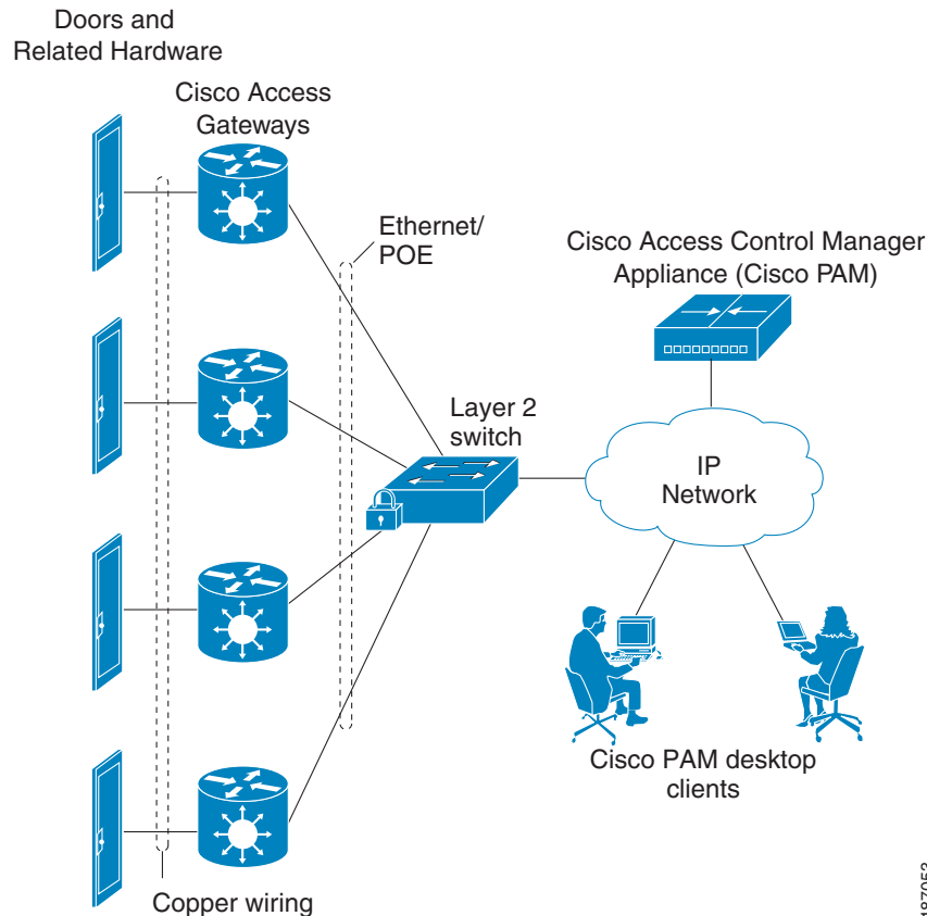
Figure 1-2 Multiple Cisco Physical Access Gateways
