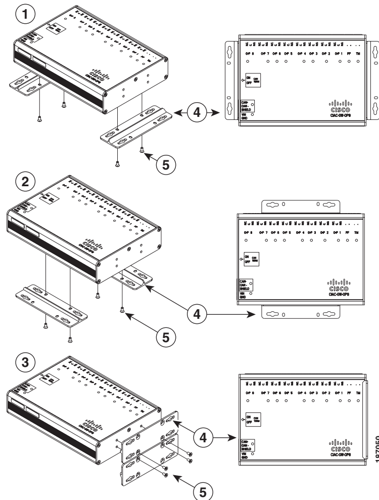
Figure 1-6 Three Options for Installing Wall Mount Brackets
