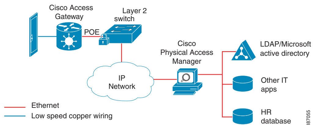
Figure 1-1 Cisco Physical Access Control: System Overview
