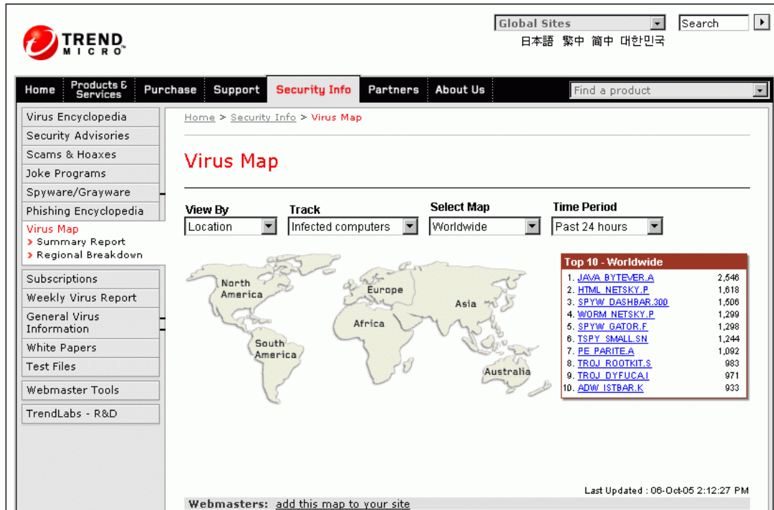
Figure 8-4 Virus Map
