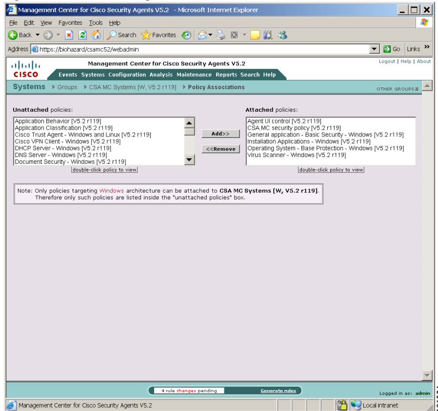
Figure 4-5 Attaching Policies
