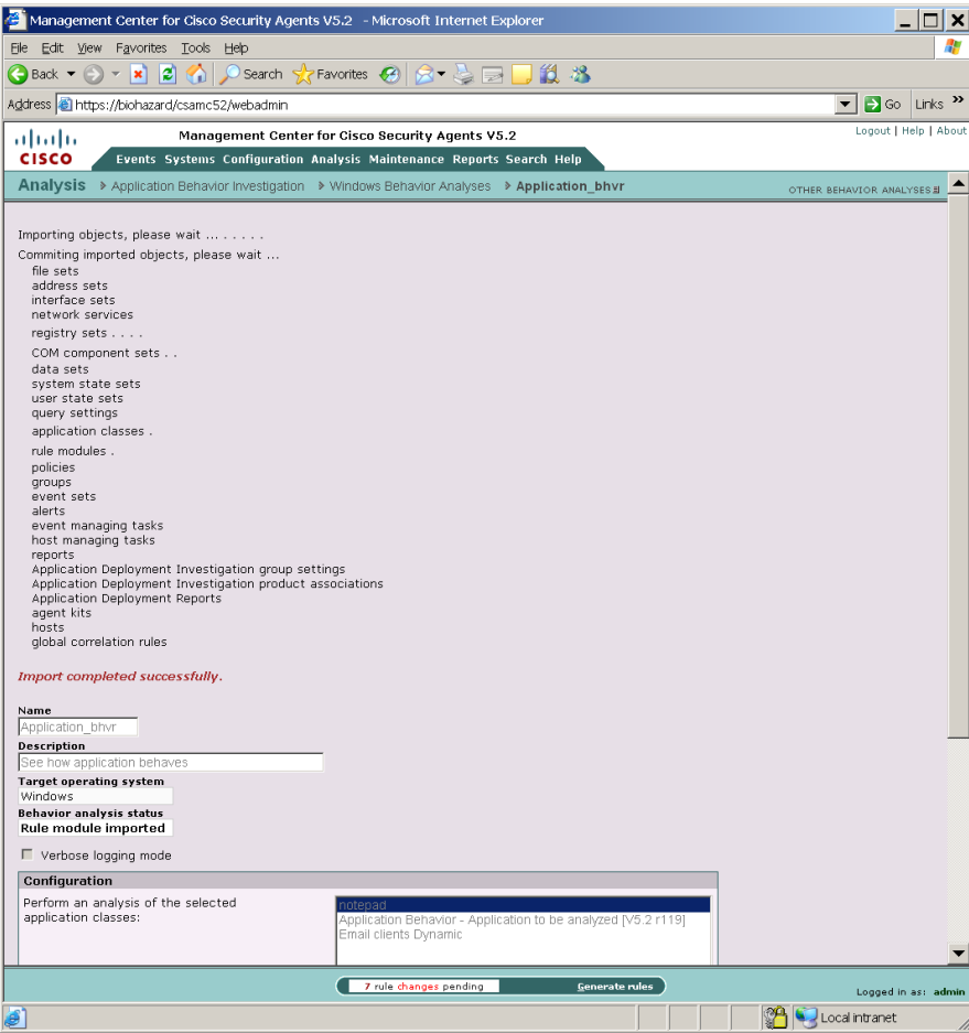
Figure 13-16 Import Process
