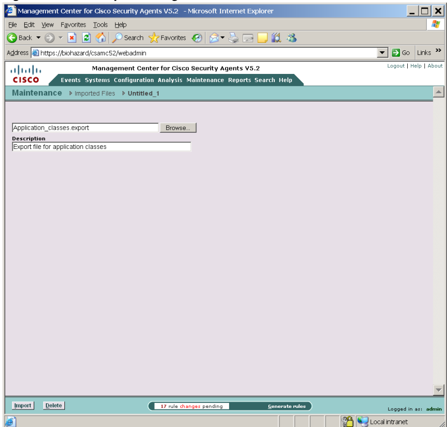
Figure 12-6 Import Configurations
