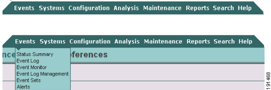
Figure 2-7 Menu Bar
