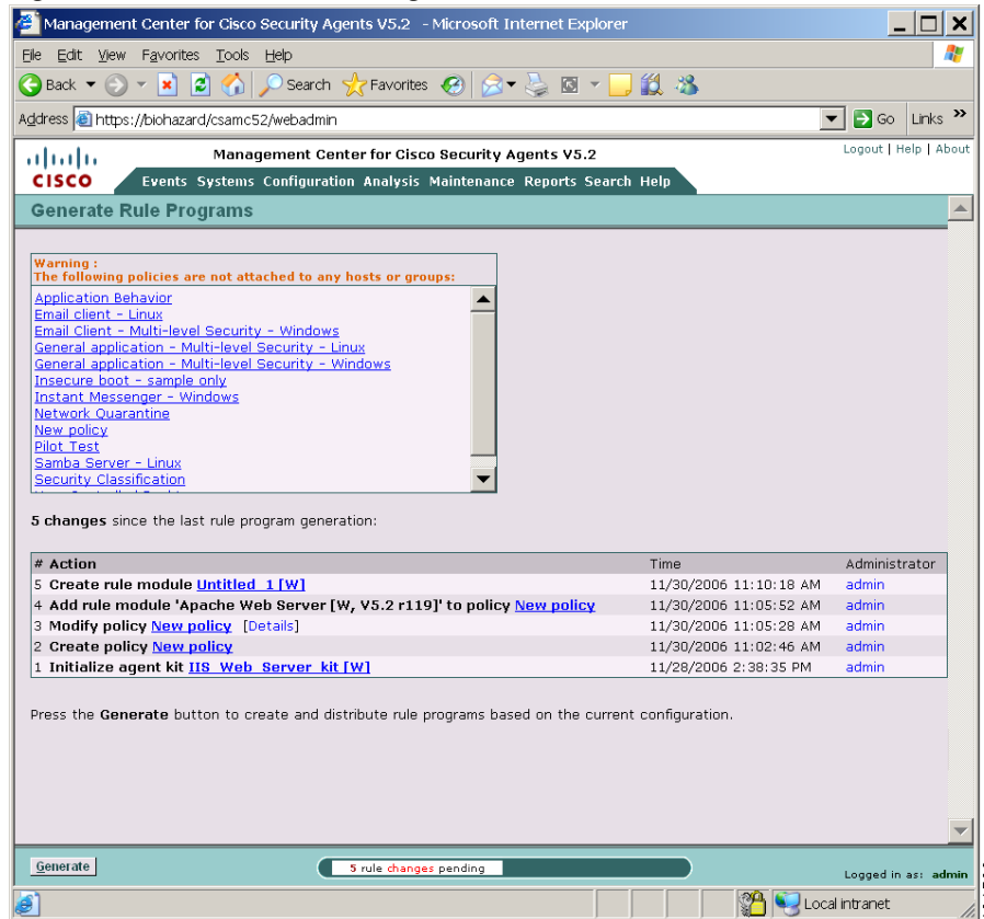
Figure 5-13 Generate Configuration
