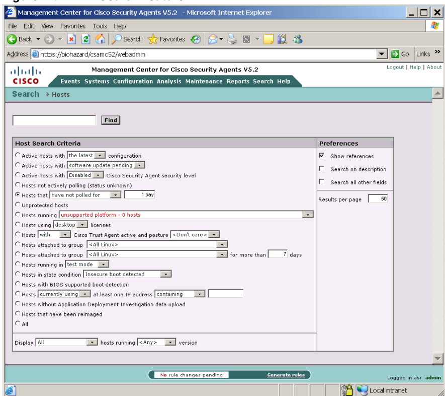
Figure 2-8 Search Feature
