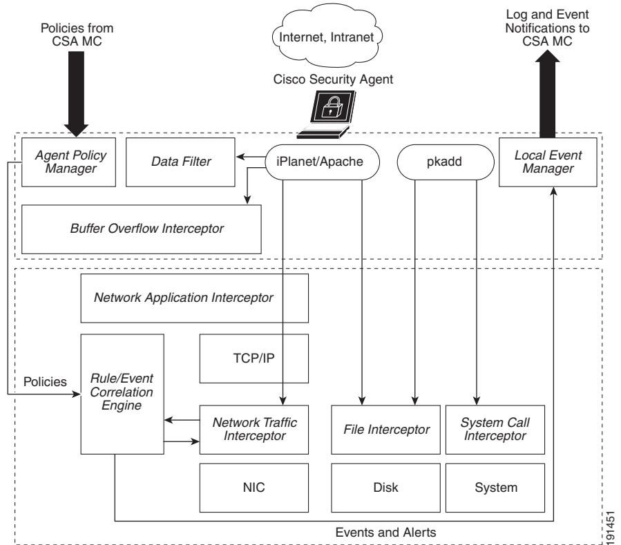
Figure B-3 Cisco Security Agent Components (UNIX) Cisco Security Agent UNIX Architecture
