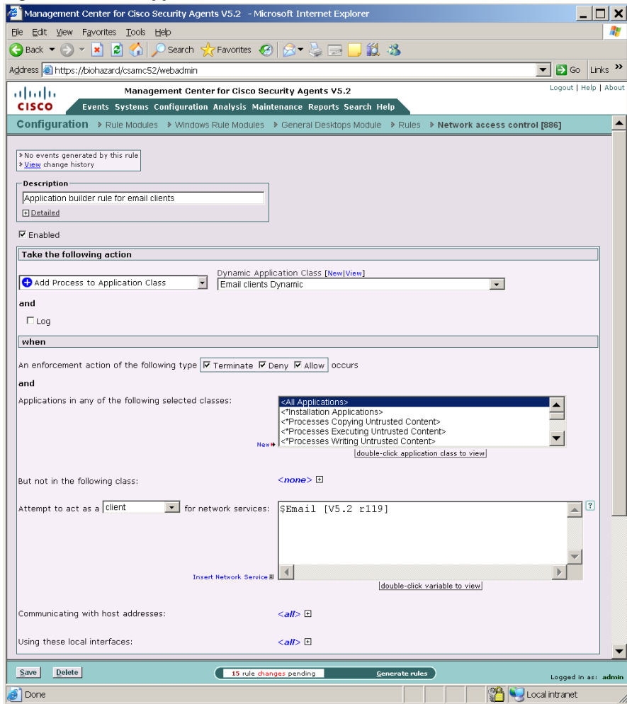
Figure 8-4 Application-Builder Rule
