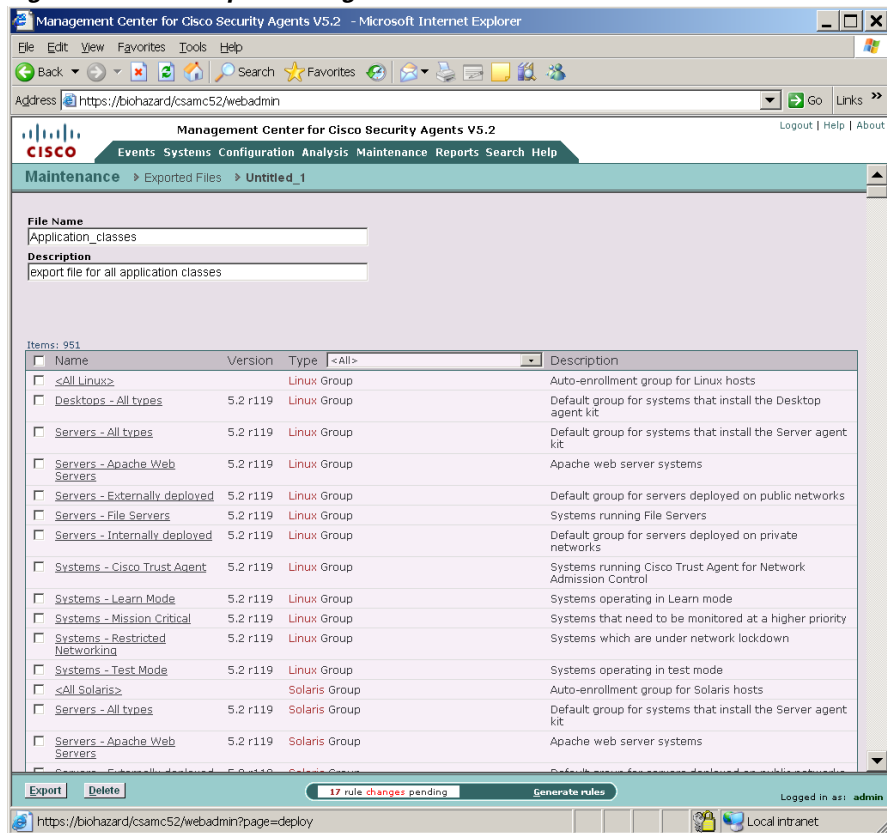
Figure 12-4 Export Configurations
