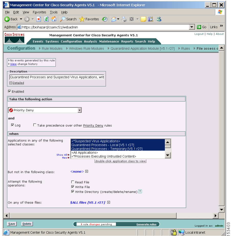
Figure 4-7 File Access Control Rule
