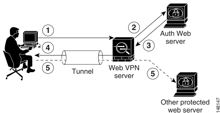
Figure 70-2 SSO Authentication Using HTTP Forms
