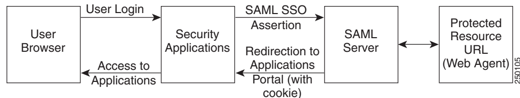
Figure 70-1 SAML Communication Flow
