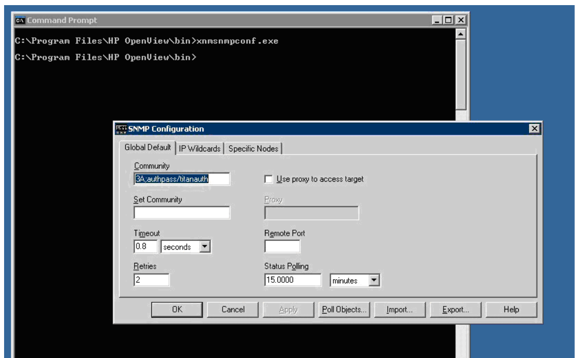
Figure 2-38 SNMP Configuration
