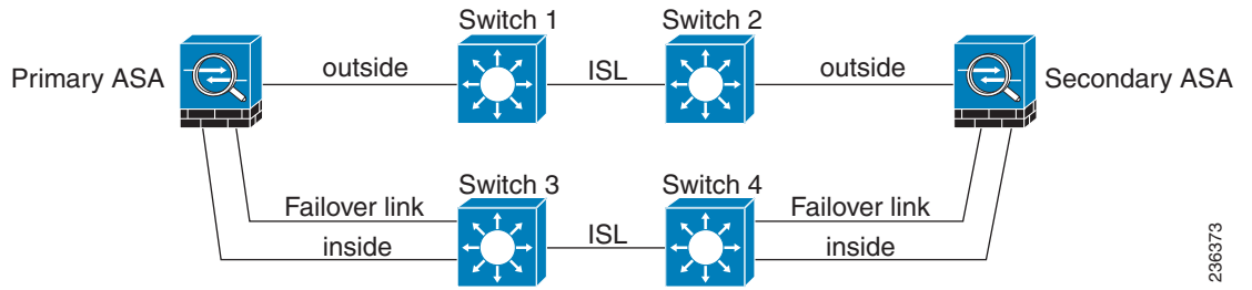
Figure 32-5 Connecting with a Secure Switch
