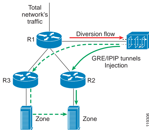
Figure A-9 Tunnel Diversion
