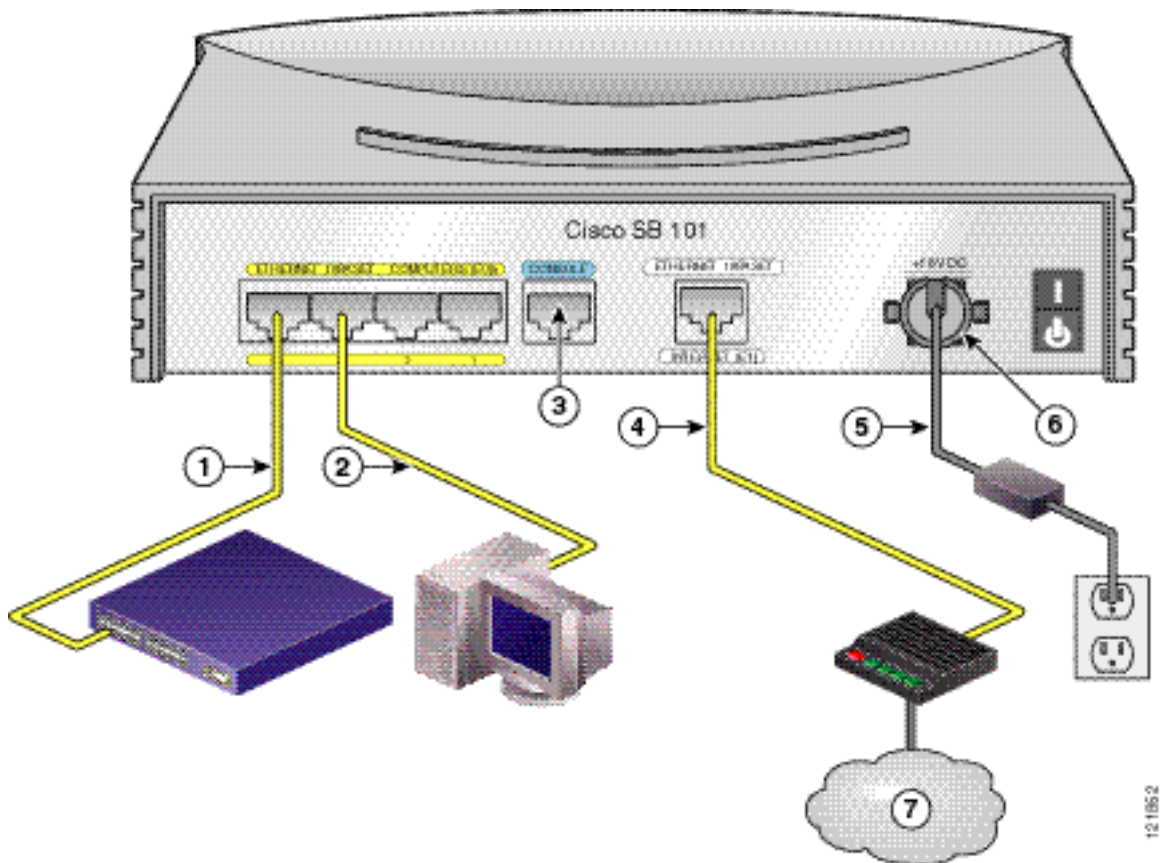
Figure 1-3 Typical Cisco SB 101 Installation
