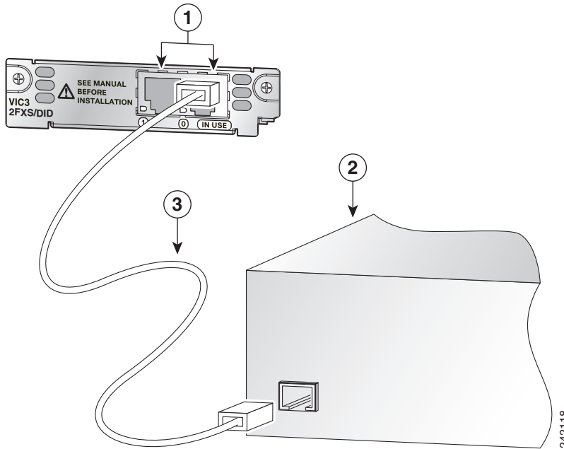
Figure 2 Cisco 2-Port FXS/DID VIC (VIC3-2FXS/DID)
