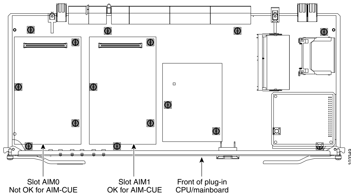
Top View of Plug-in CPU/Mainboard in Cisco 3745 Router
