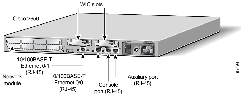
Figure 2 Cisco 2621XM and Cisco 2651XM Physical Interfaces
