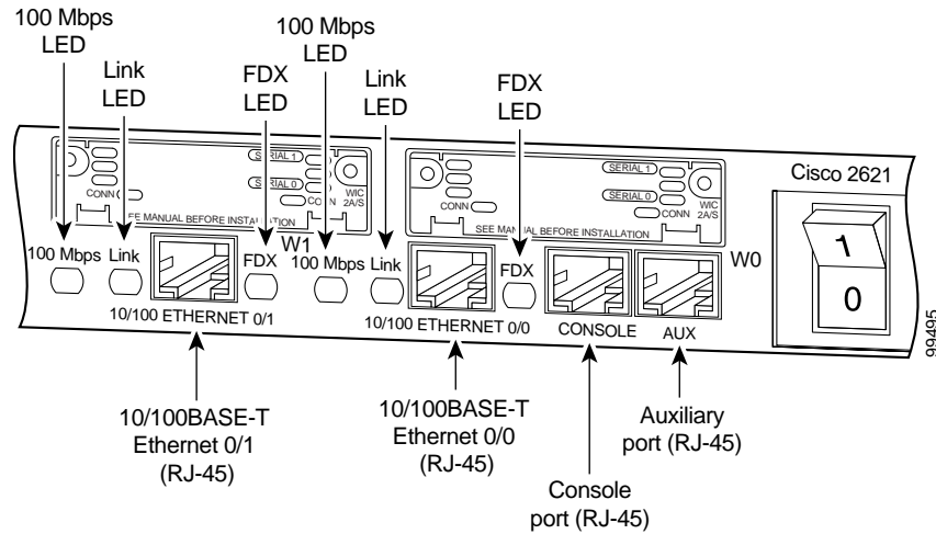
Figure 3 Cisco 2621XM and Cisco 2651XM Rear Panel LEDs
