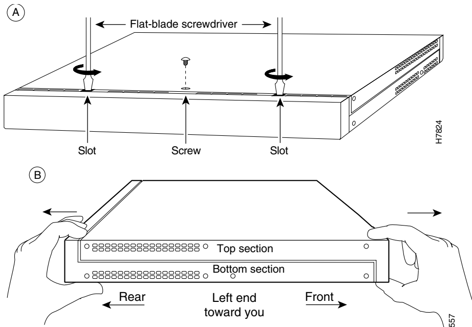
Figure B-1 Chassis Cover Removal
