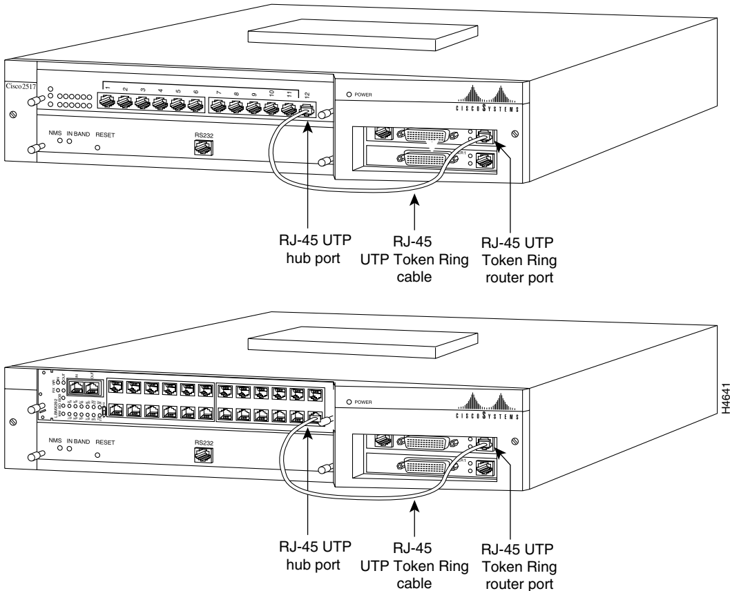
Figure 3-3 Connecting the Router Card to the Hub Port Card
