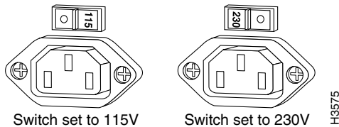
Figure 3-4 Power Supply Input Voltage Selection Switch
