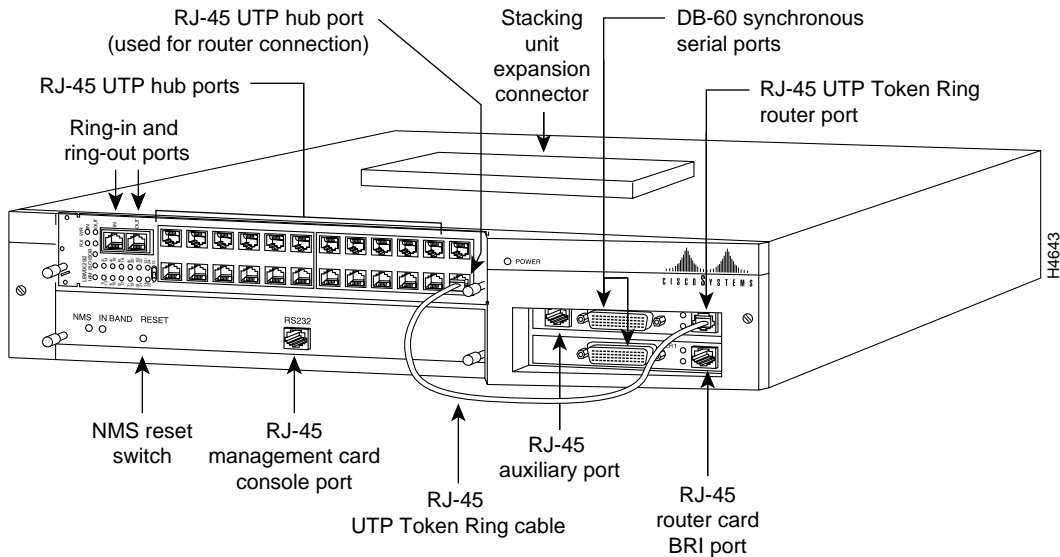
Figure 1-2 Cisco 2519 24-port Router/Hub
