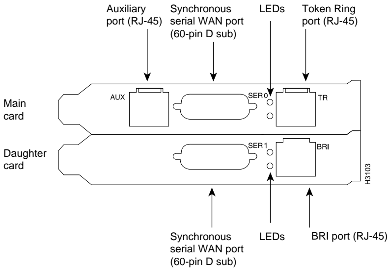
Figure 1-9 Token Ring Router Card Ports
