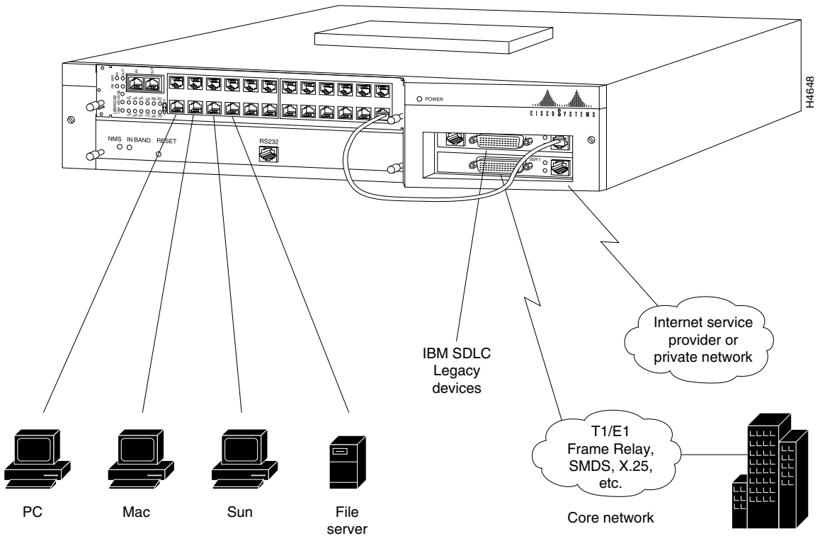
Figure 5-2 Asynchronous Routing
