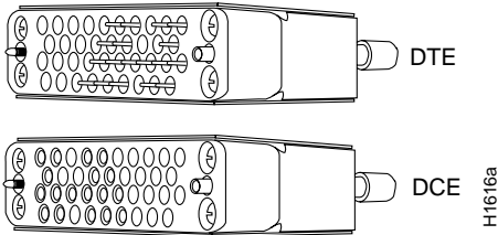
Figure 2-4 V.35 Serial Transition Cable Connectors, Network End
