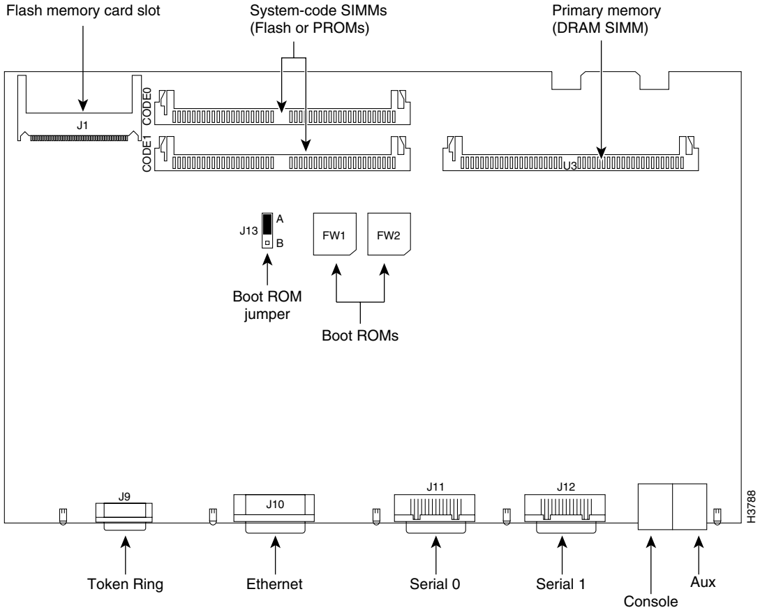
Figure B-3 System Card Layout—Model 2513 Router
