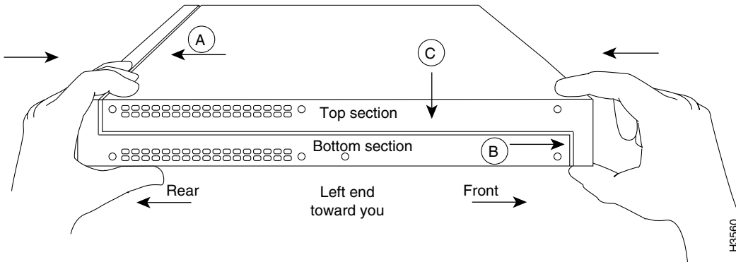
Figure B-8 Replacing the Chassis Cover
