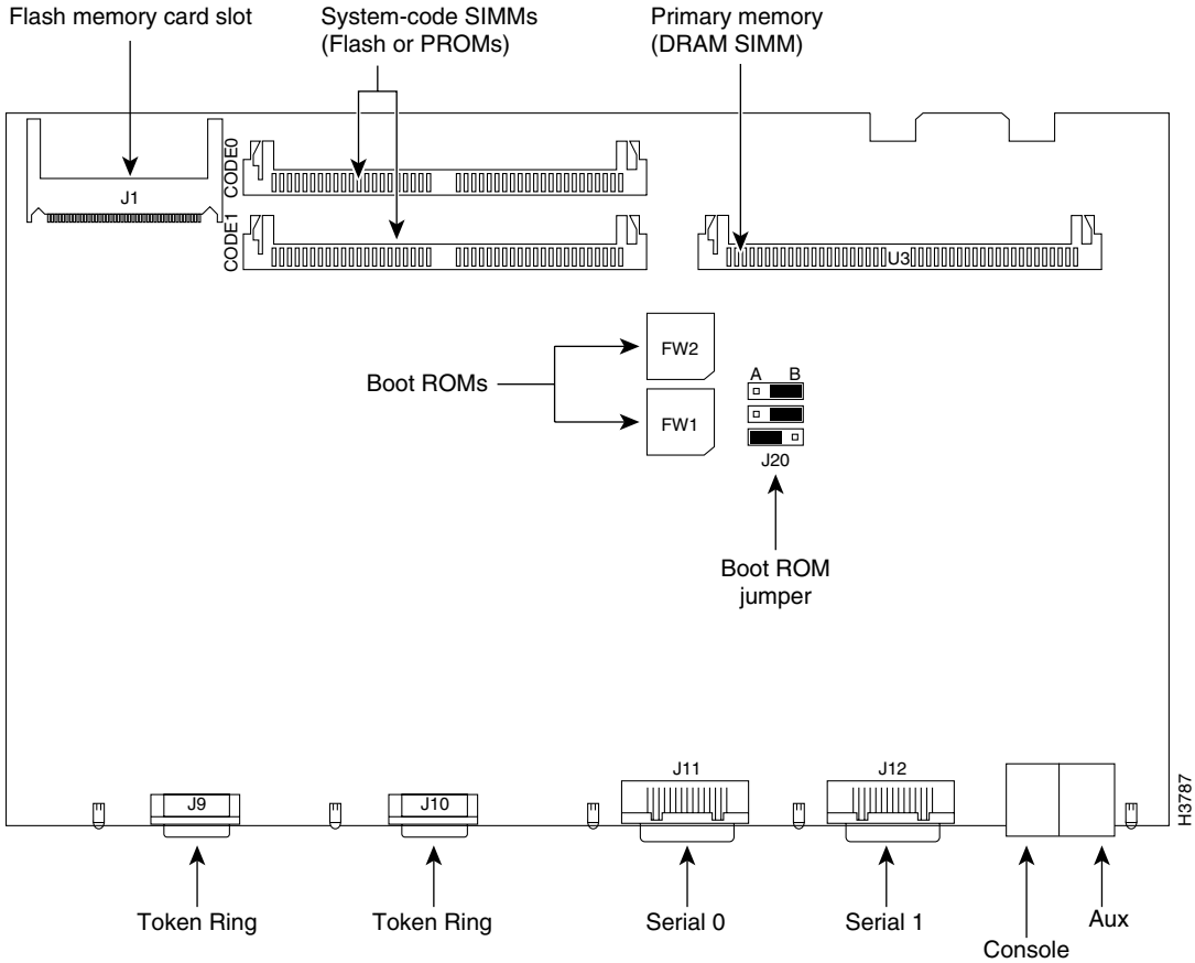
Figure B-5 System Card Layout—Model 2515 Router
