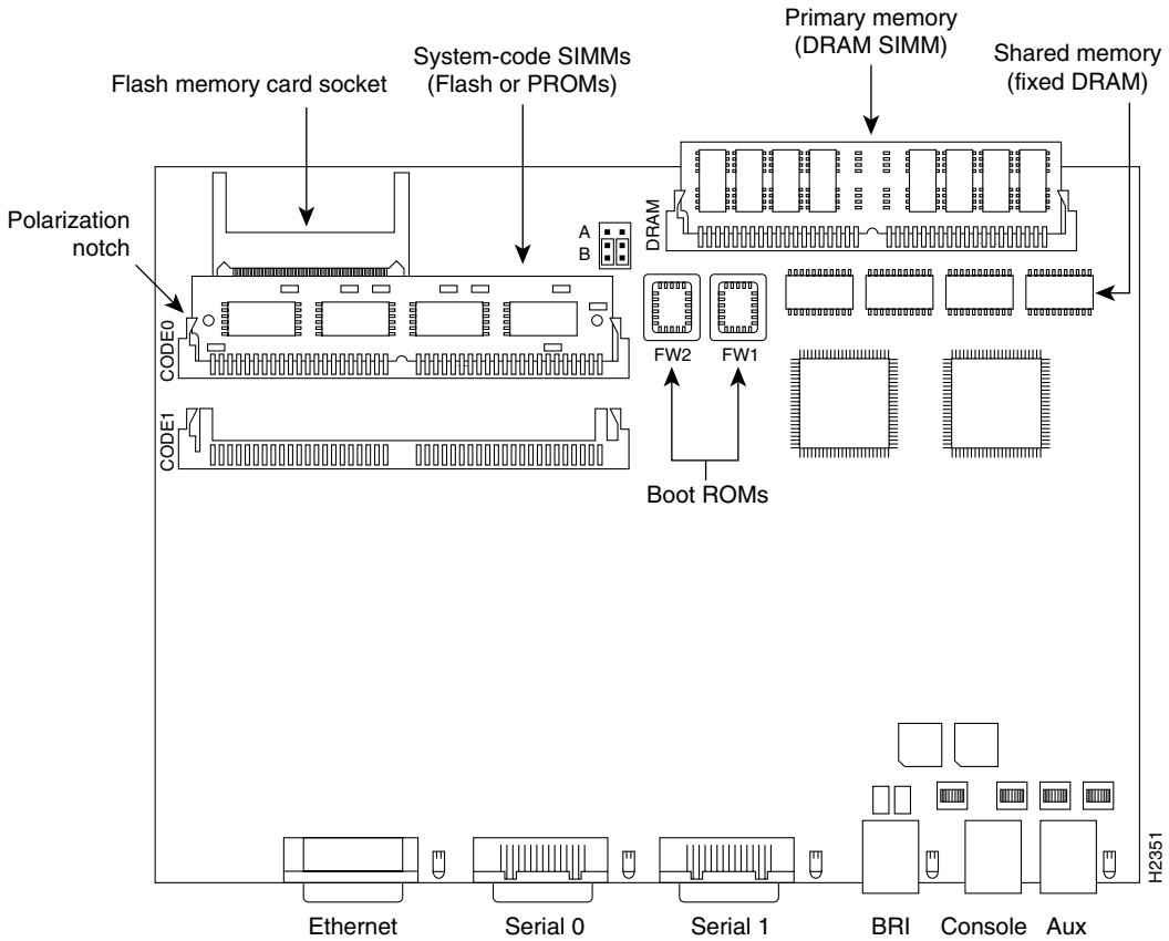
Figure B-2 System Card Layout—Model 2501, 2502, 2503, and 2504 Routers
