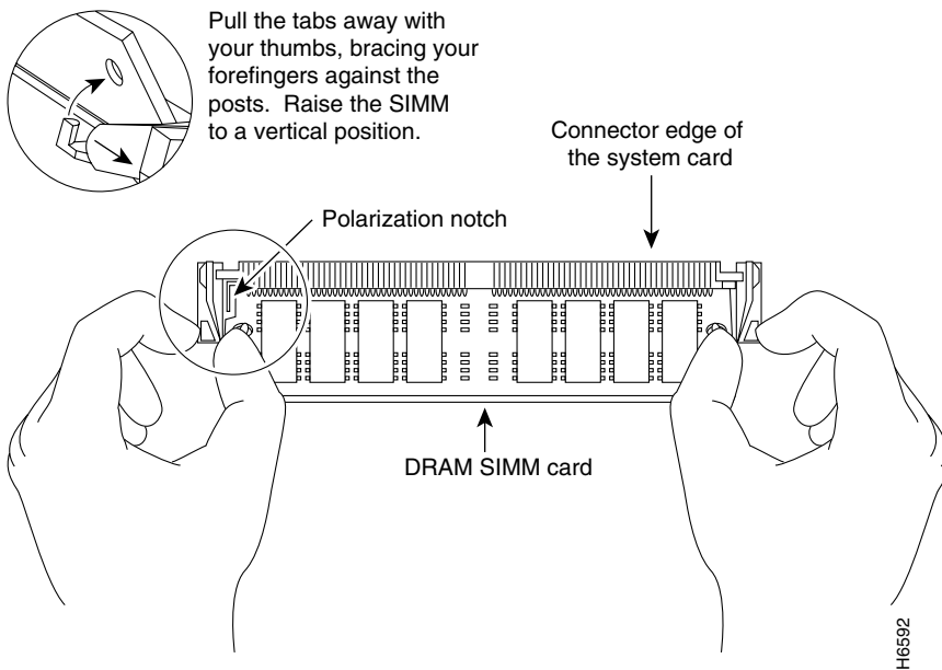
Figure B-6 Removing and Replacing the DRAM SIMM
