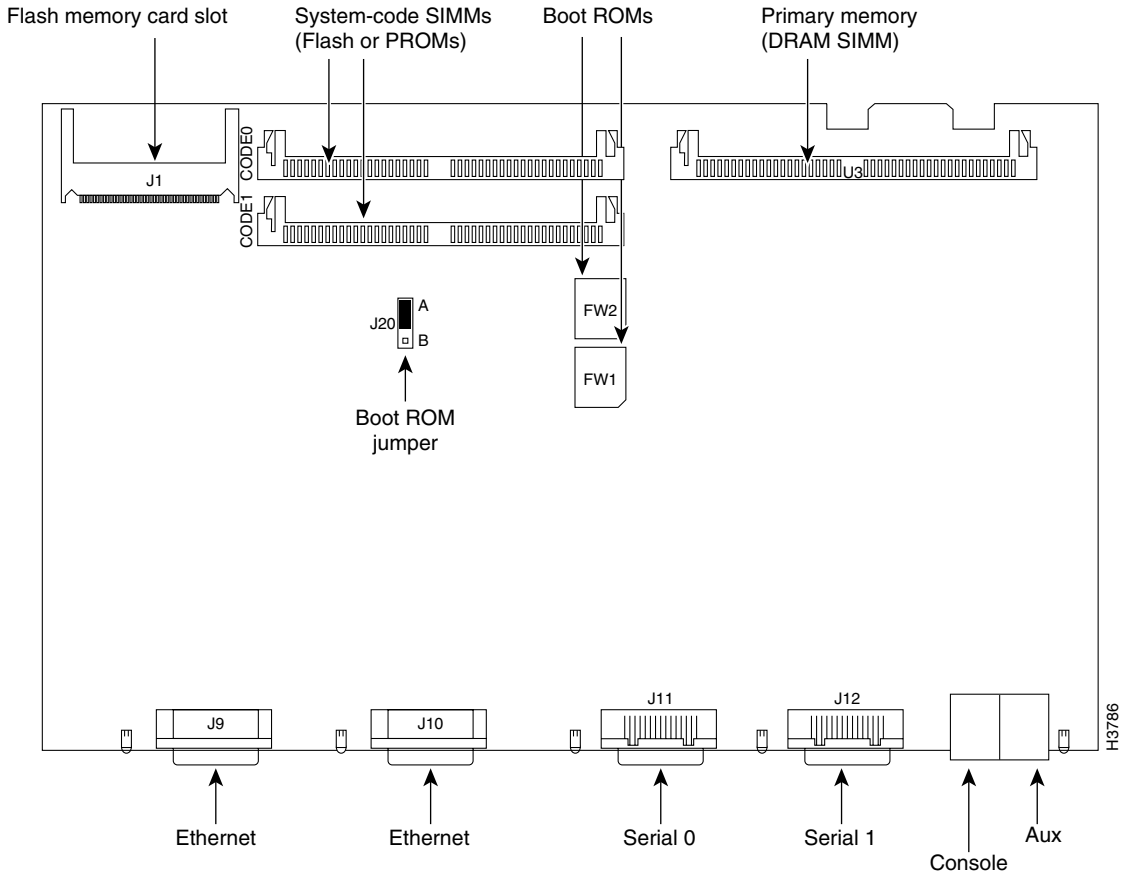
Figure B-4 System Card Layout—Model 2514 Router
