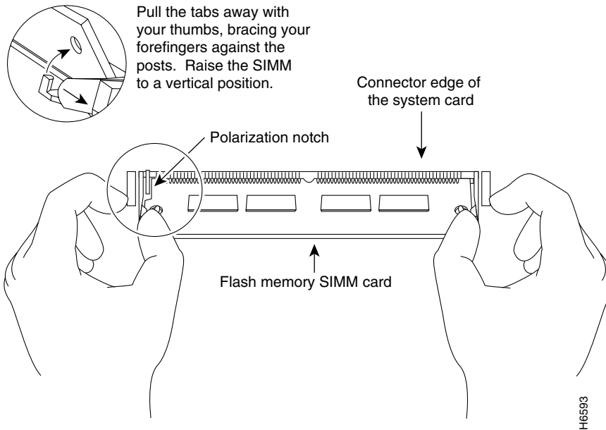
Figure B-7 Removing and Replacing the System-Code SIMM
