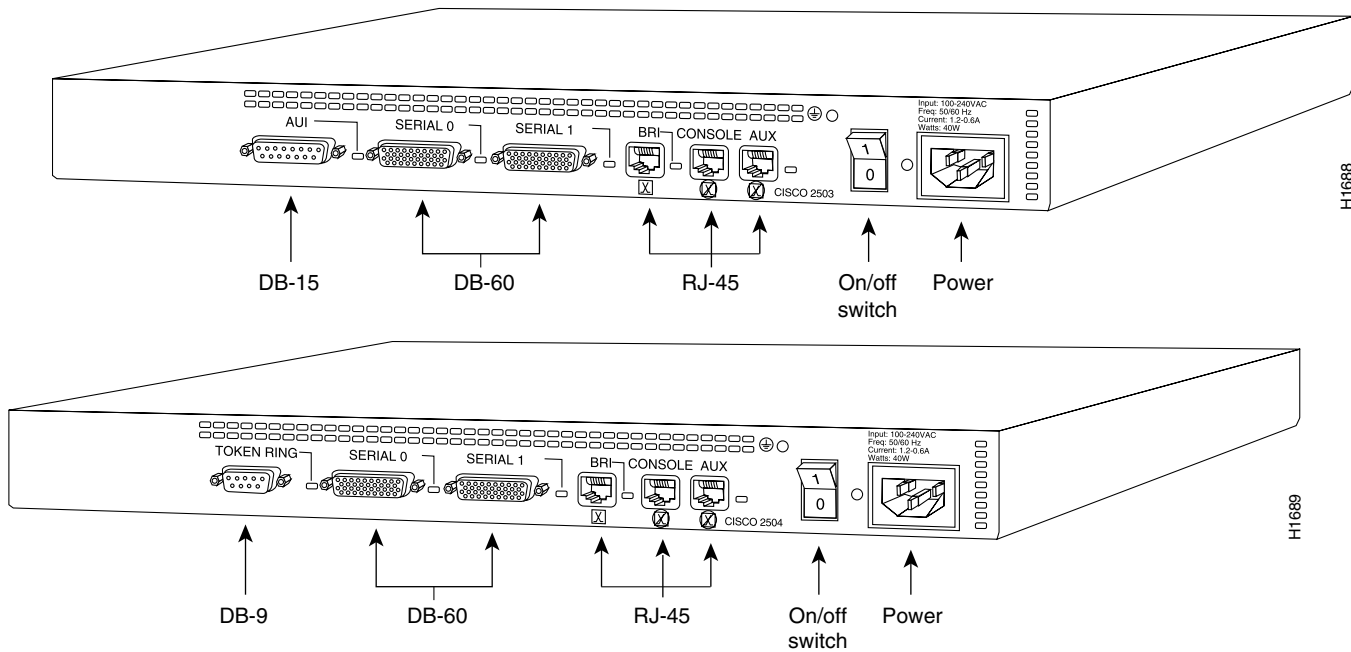
Figure 1-2 Router Rear View—Models 2503 and 2504
