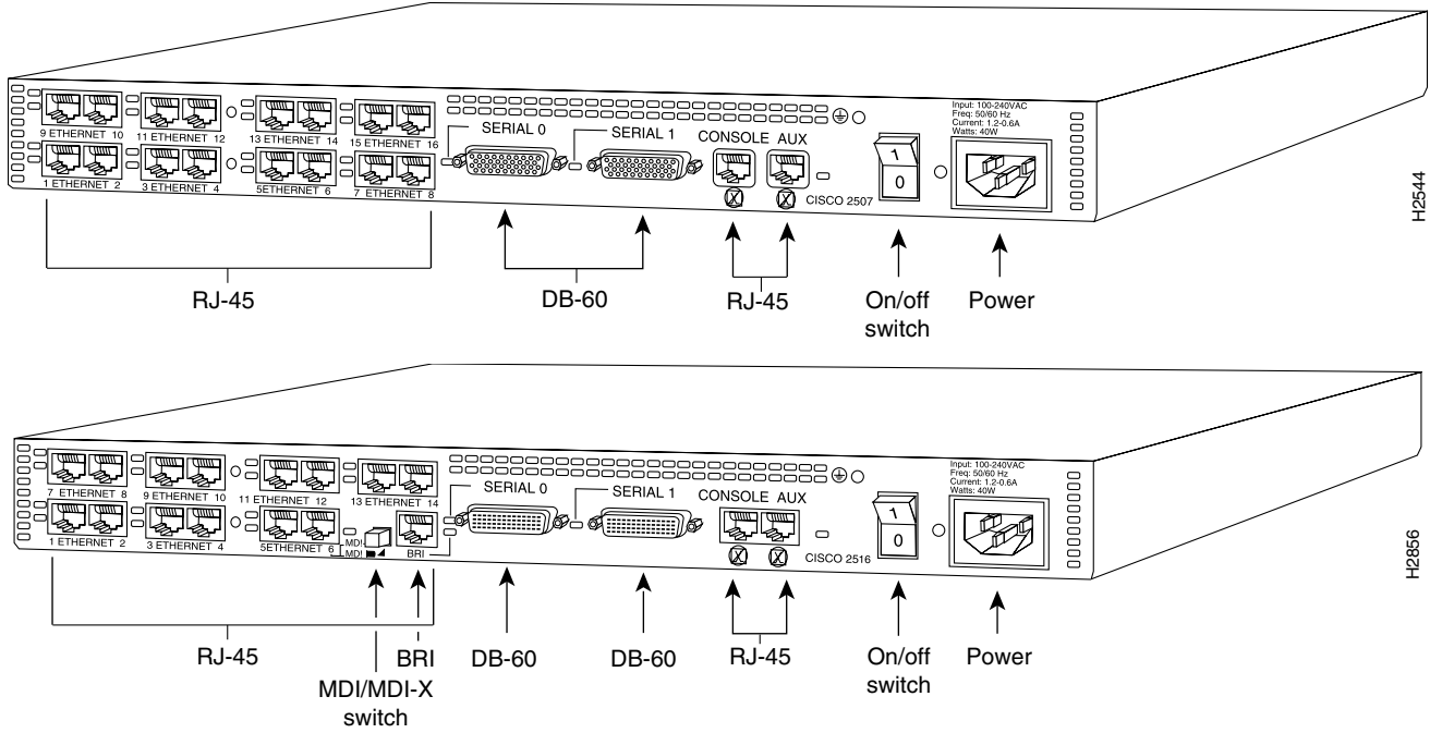
Figure 1-3 Hub Rear View — Models 2507 and 2516
