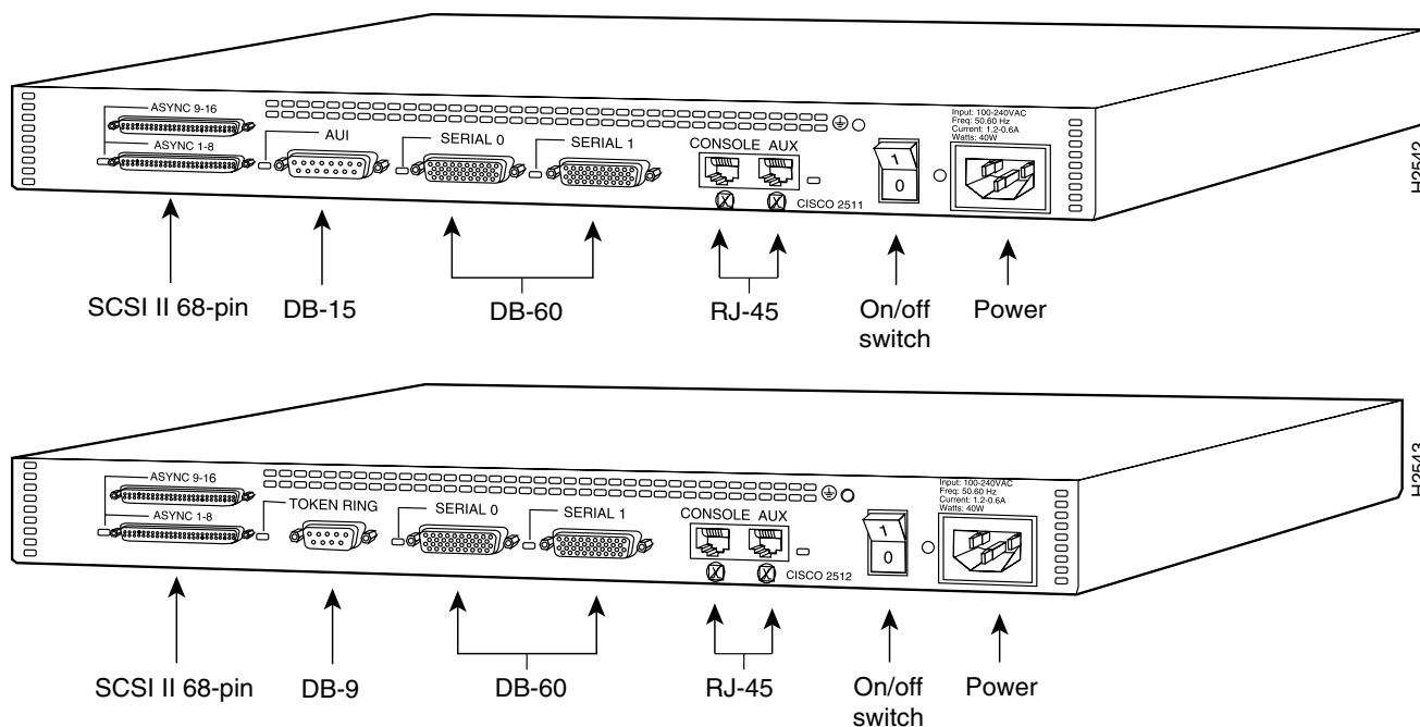
Figure 1-4 Access Server Rear View — Models 2511 and 2512
