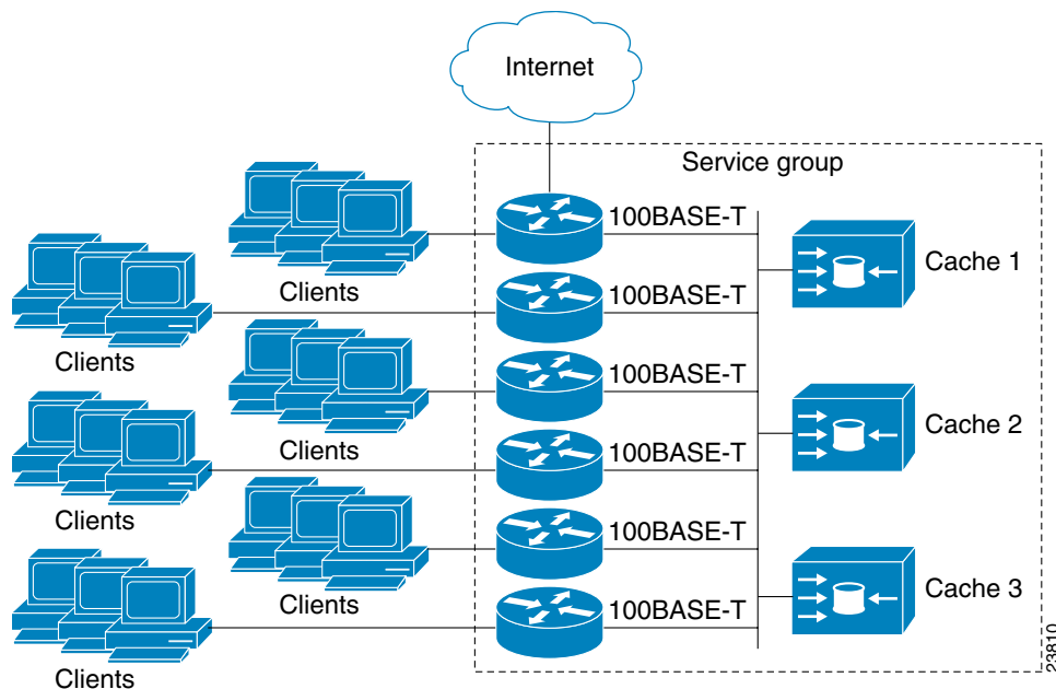
Figure 56-2 Cisco Cache Engine Network Configuration Using WCCP v2
