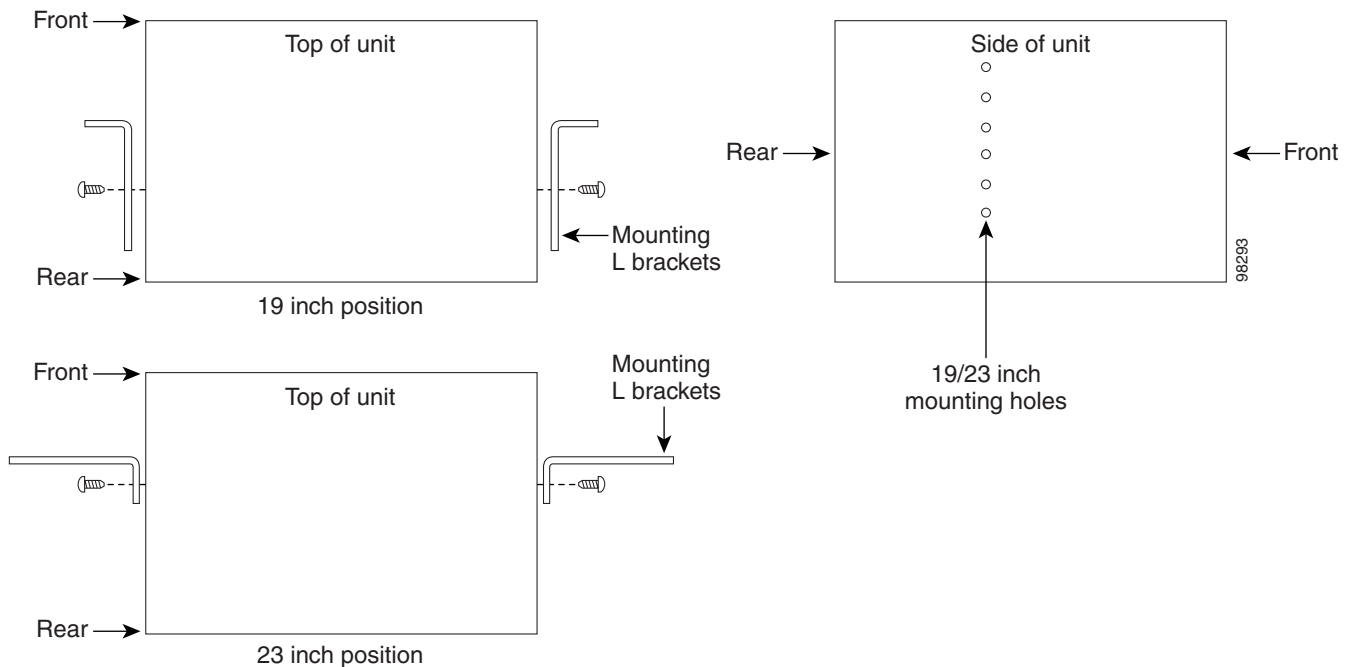
Figure 1 Positioning the mounting brackets
