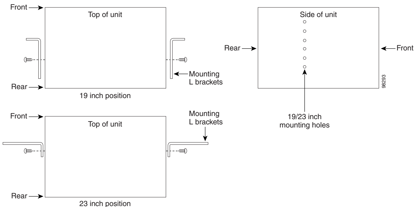
Figure 1 Positioning the mounting brackets
