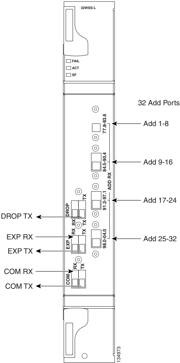
Figure 10-4 32WSS-L Faceplate and Ports
