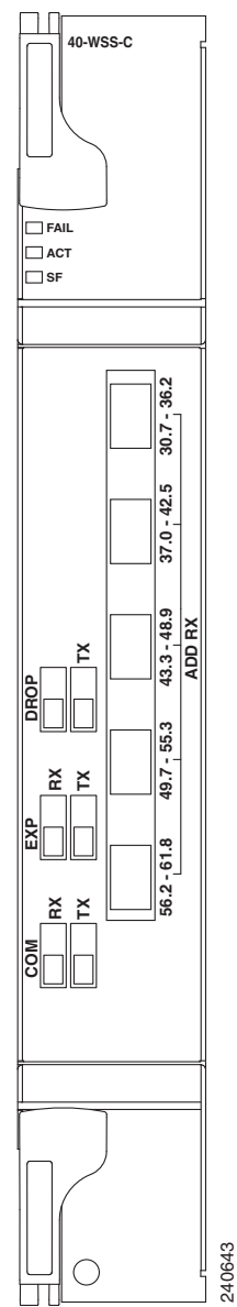
Figure 10-25 40-WSS-CE Faceplate
