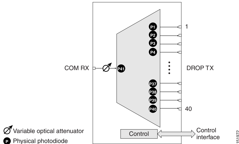
Figure 10-15 40-DMX-C Optical Module Functional Block Diagram
