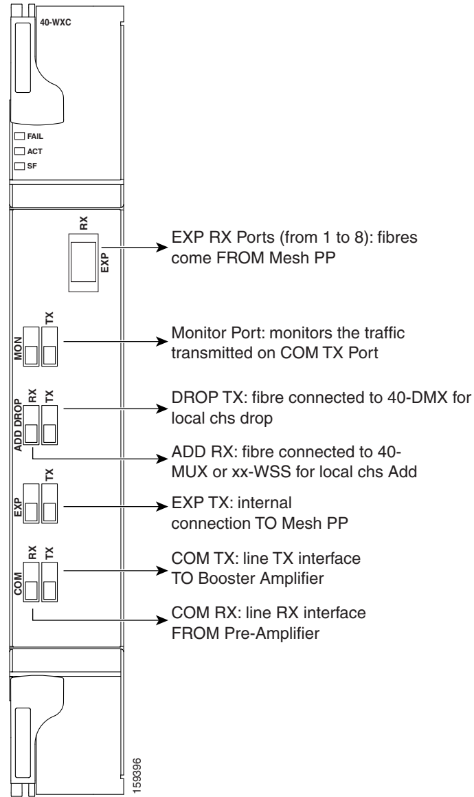
Figure 10-28 40-WXC-C Faceplate
