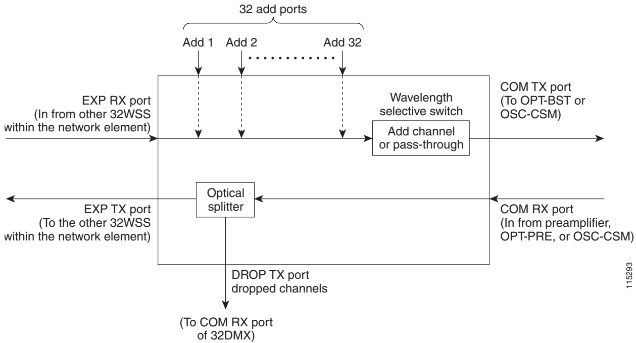
Figure 10-2 32WSS Block Diagram
