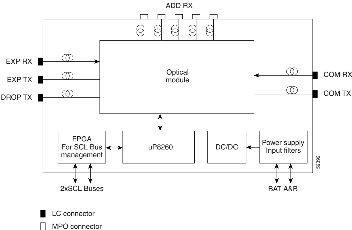
Figure 10-27 40-WSS-CE Card Optical Module Functional Block Diagram
