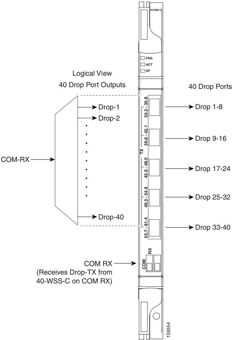
Figure 10-13 40-DMX-C Faceplate
