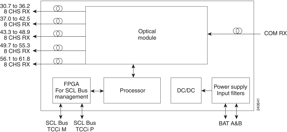
Figure 10-17 40-DMX-CE Card Block Diagram
