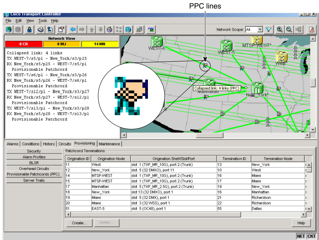
Figure 16-6 Viewing the Provisionable Patchcords Table
