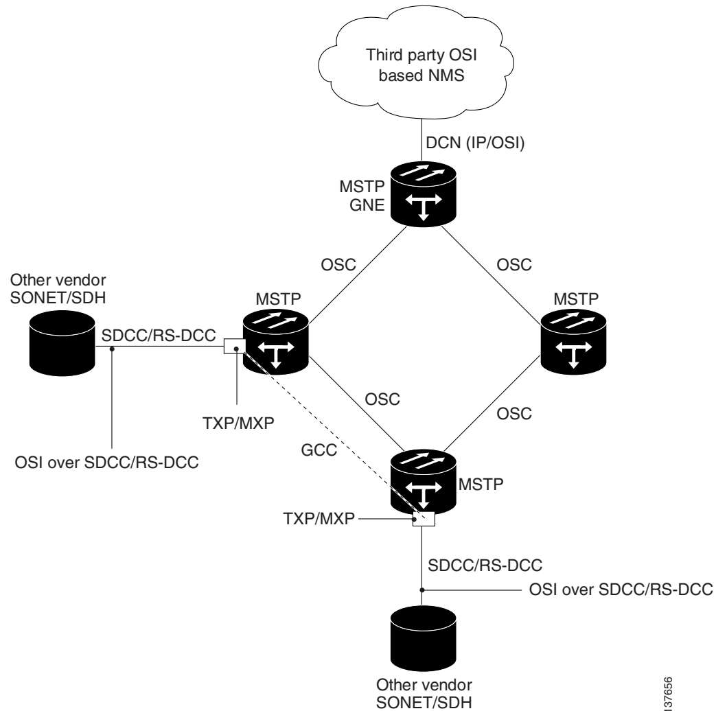
Figure 22-27 OSI/MSTP Scenario 1
