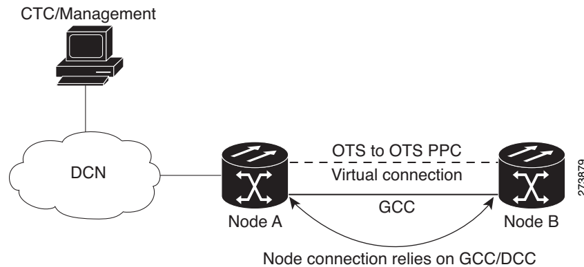
Figure 22-24 Network Using GCC/DCC
