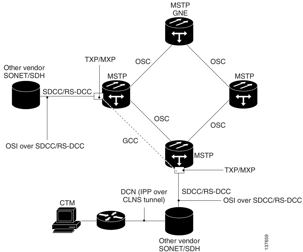
Figure 22-30 OSI/IP Scenario 4
