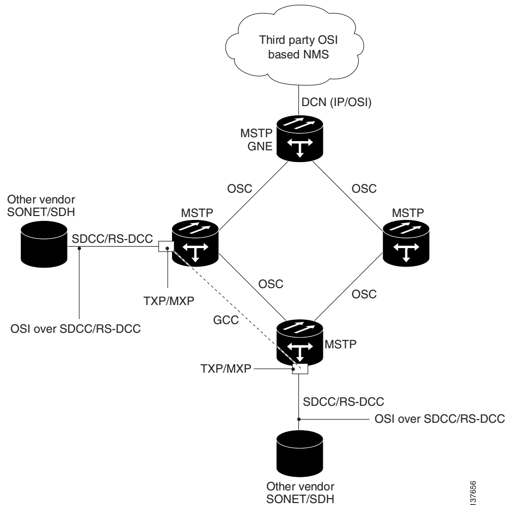
Figure 22-27 OSI/MSTP Scenario 1
