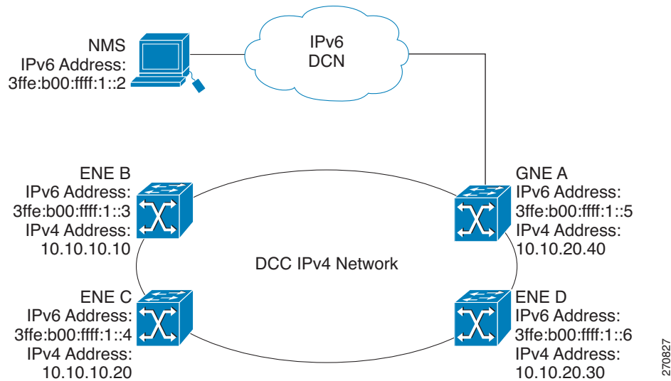
Figure 22-33 IPv6-IPv4 Interaction
