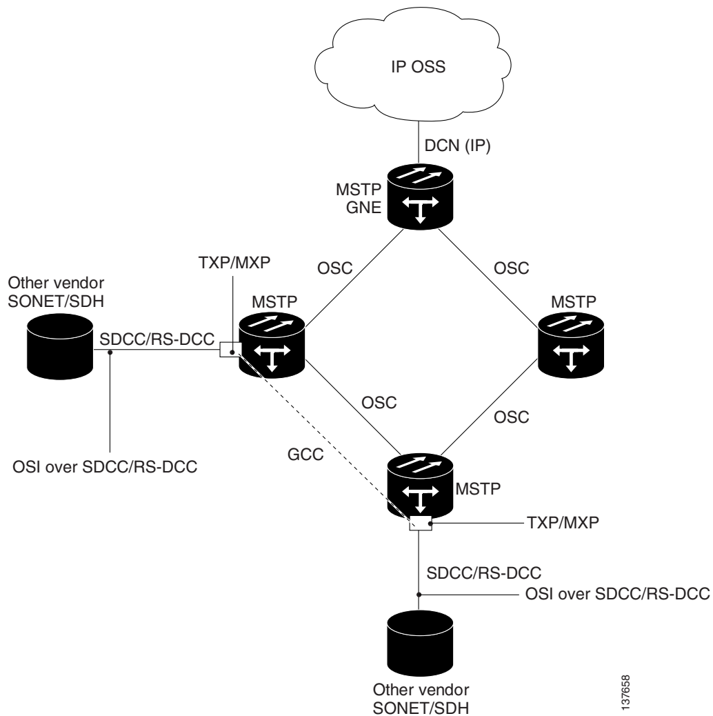
Figure 22-29 OSI/MSTP Scenario 3
