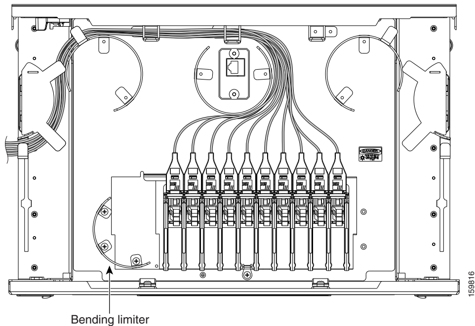
Figure 4-21 40-Channel Patch Panel Tray, Top View
