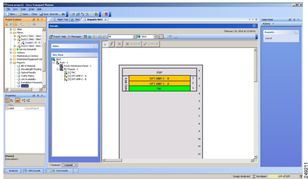
Figure 4-2 Cisco Transport Planner shelf layout - ONS 5454 M2
