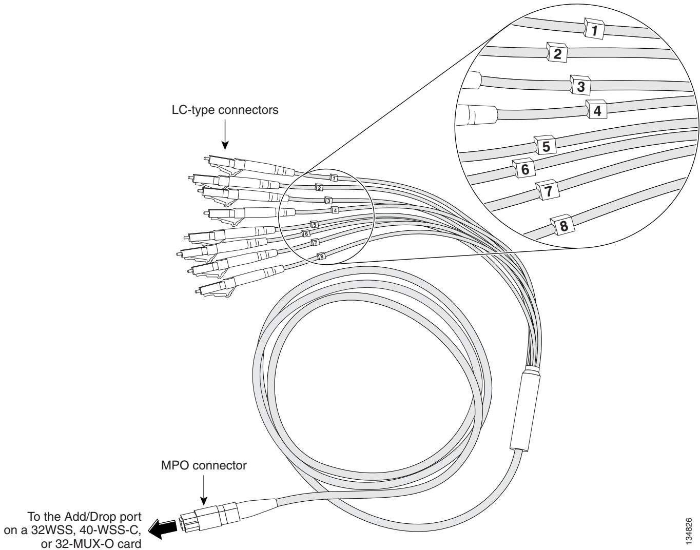
Figure 4-14 MPO Cable
