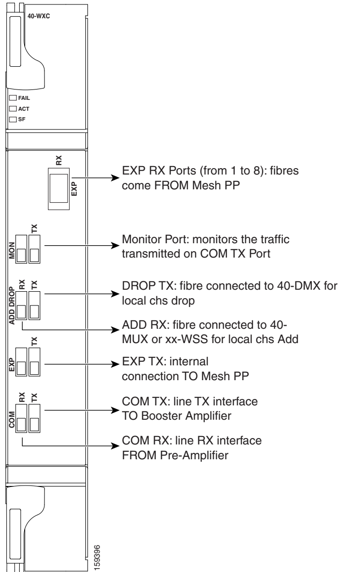
Figure 9-34 40-WXC-C Faceplate
