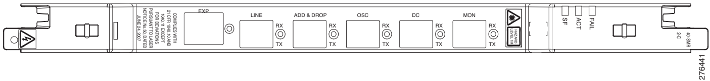
Figure 9-39 40-SMR2-C Faceplate
