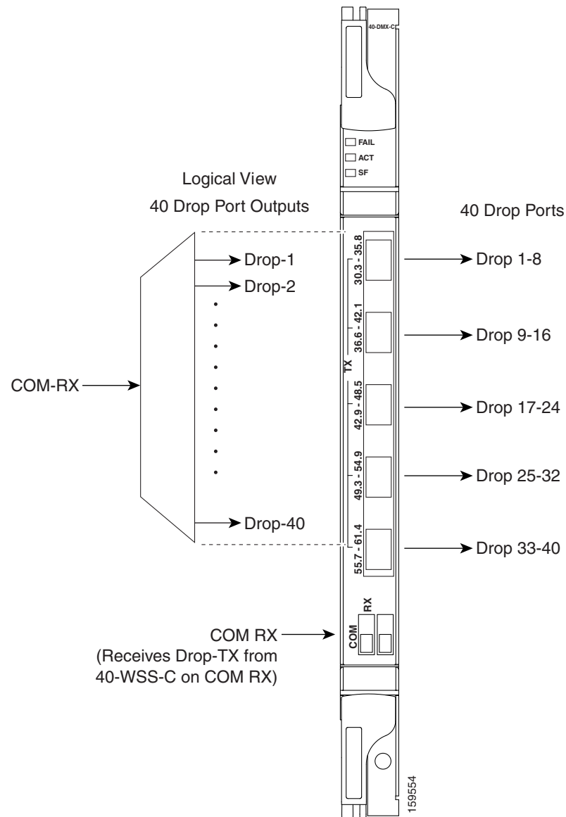
Figure 9-19 40-DMX-C Faceplate
