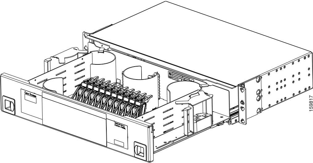
Figure 1-46 40-Channel Patch-Panel Tray, Side View
