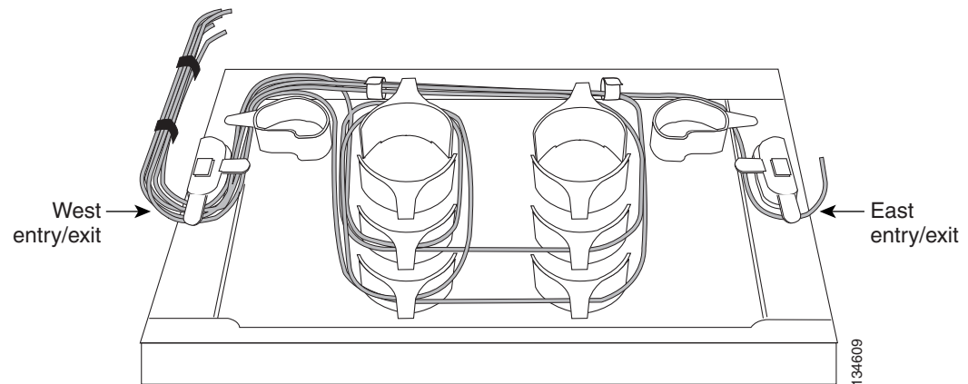
Figure 1-51 Fiber-Storage Tray
