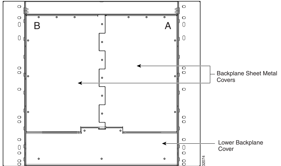
Figure 1-27 Backplane Covers
