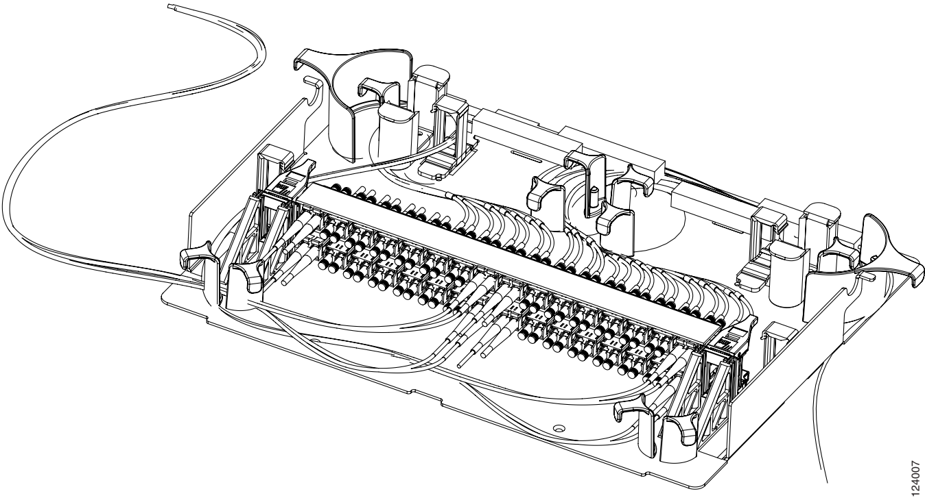
Figure 1-43 Standard Patch-Panel Tray
